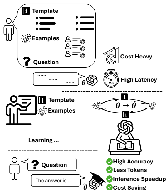
Figure 1: An illustration of PromptIntern: Like human interns, LLMs learn and internalize repeated prompt information such as templates and examples during fine-tuning, leading to efficient and effective inference.
