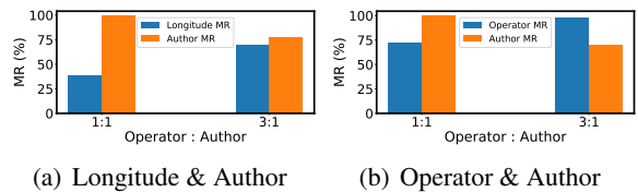
Figure 9: The effect of frequency for fact memorization.
