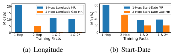
Figure 7: LLM memorization for derivable facts, where “*” means that facts are from another group of keys.
