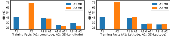
Figure 16: Supplementary results of memorization on correlated facts, where “*” means that facts are from another group of keys.
