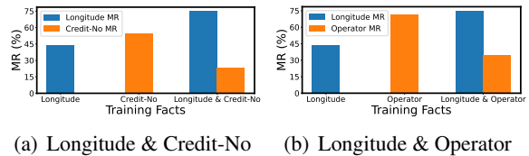
Figure 10: The effect of difficulty for fact memorization.
