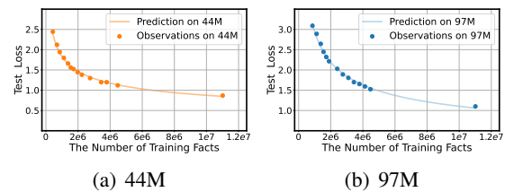
Figure 11: LLMs’ fact generalization loss across different numbers of training facts.
