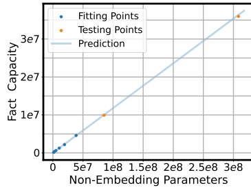
(b) 200 Epochs
