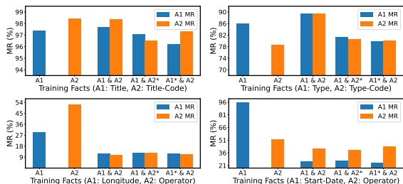
Figure 6: Memorization on correlated facts, where “*” means that facts are from another group of keys.
