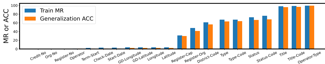
Figure 12: Memorization and generalization over facts of different types, on 44M LLM trained by 10M facts.
