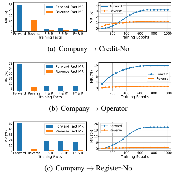
Figure 5: LLMs’ memorization of the same facts with different directions, where “*” means facts are from another group of keys. The right is the learning curves.
