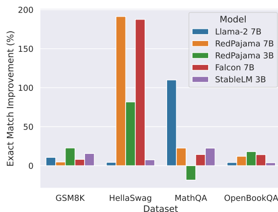
Figure 1: Percentage of improvement using the best loss function for each task (on average, Lovász loss for GSM8K and MathQA, and Focal loss for HellaSwag and OpenBookQA) combined with Cross-Entropy compared to model fine-tuned with Cross-Entropy only.
