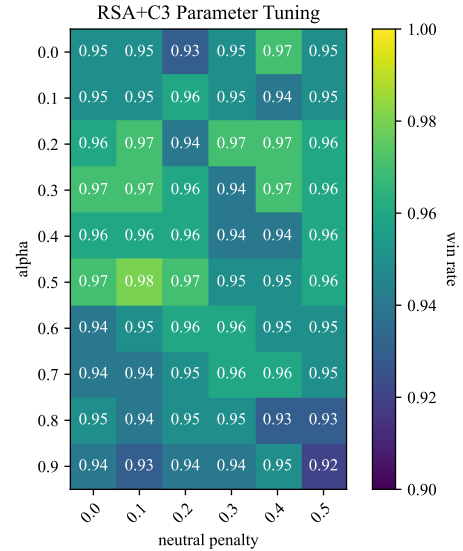
Figure 9: Hyperparameter Tuning for RSA+C3 across the axes of alpha and neutral penalty. We find that a neutral penalty of 0.1 and an alpha of 0.5 performed the best.
