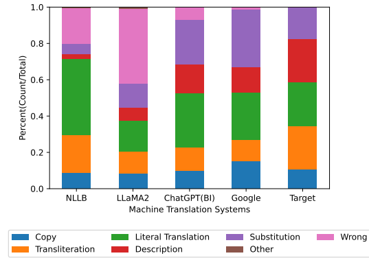
Figure 9: Percentage of translation strategies.
