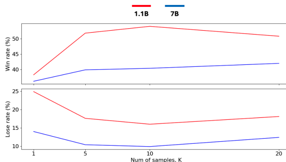
Figure 5: Impact of varying K to approximate the average contradiction score. The value of K affects the number of responses used to compute both S_L and S_K .
