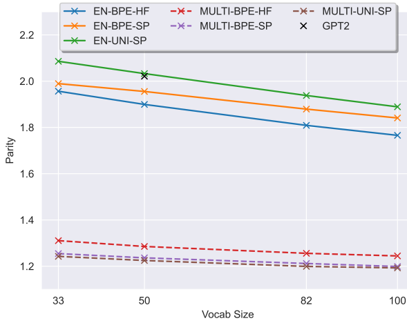
Figure 2: Comparison of parity scores between mono-lingual (English) tokenizers and multilingual tokenizers applied to multilingual documents.
