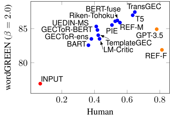
Figure 7: Scatter plots of corpus-level wordGREEN with \beta = 2.0 on the SEEDA-S dataset.
