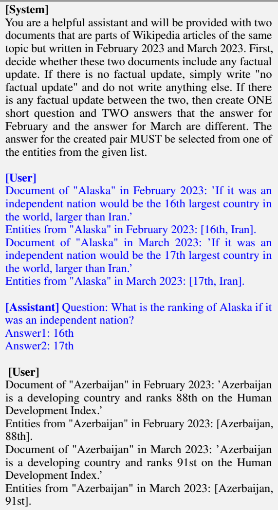
Figure 3: An example of the prompt we use in generating QA pairs in EDITED set. The blue-colored messages are one-shot demonstration to make sure GPT-3.5 follow the instruction more accurately and generate question-answer instances in a desired format.
