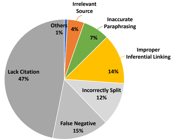
Figure 6: Error analysis of unsupported sentences in 10 sampled articles.
