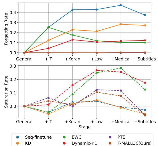
Figure 4: Forgetting rate and saturation rate across different training stages.
