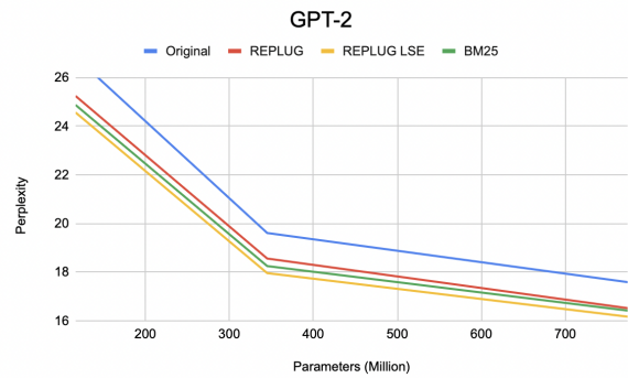
Figure 8: PPL of GPT-2 models on Wikitext-103 with no retrieval (Origin), Contriever (REPLUG), LM-supervised Contriever (REPLUG LSR) and BM25.
