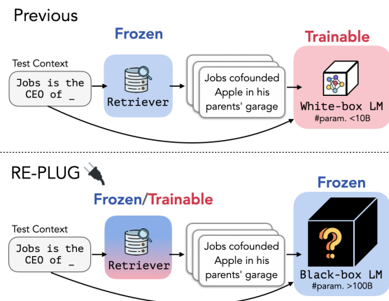
Figure 1: Different from previous retrieval-augmented approaches (Borgeaud et al., 2022) that enhance a language model with retrieval by updating the LM’s parameters, REPLUG treats the LM as a black box and augments it with a frozen or tunable retriever. This black-box assumption makes REPLUG applicable to large LMs, which are often served via APIs.
