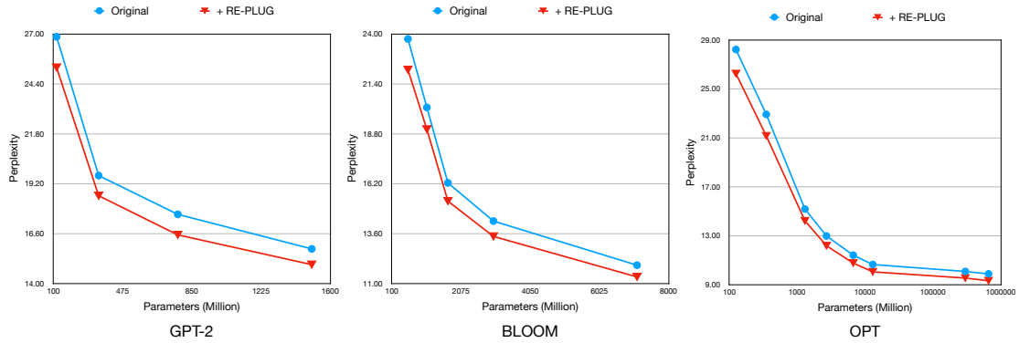
Figure 4: GPT-2, BLOOM and OPT models of varying sizes consistently benefit from REPLUG. The x-axis indicates the size of the language model and the y-axis is its perplexity on Wikitext-103.
