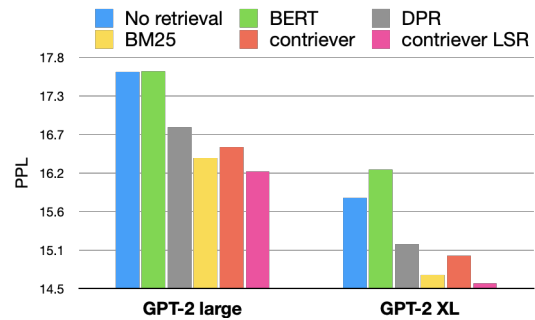
Figure 6: LM-supervised retriever (Contriever LSR) outperforms other off-the-shelf retrievers.
