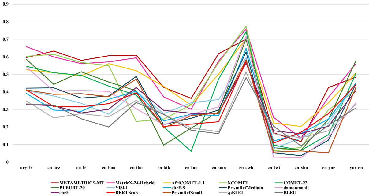
Figure 4: Spearman-rank Correlations of MT Evaluation Metrics for each language pair.
