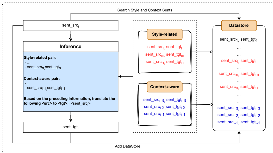
Figure 2: The overall of our incremental decoding framework.
