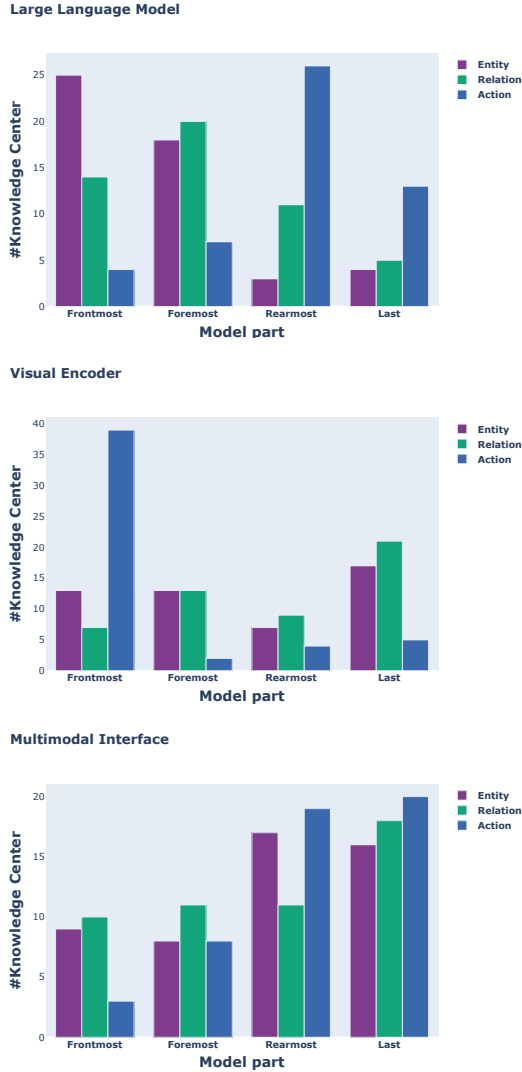
Figure 5: The distribution of the layers that need to be edited for the knowledge centers in the four parts of MLLM components.
