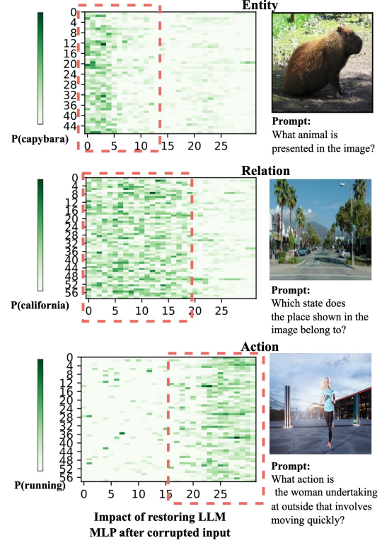
Figure 4: Causal Tracing Results for the LLM MLP of MLLM. The horizontal axis represents different layers, while the vertical axis represents the input characters. The intensity of the bars indicates the probability of generating the correct answer (after causal intervention). Knowledge of different granularities (i.e., entity, relation, action) is scattered in different layers in the LLM.
