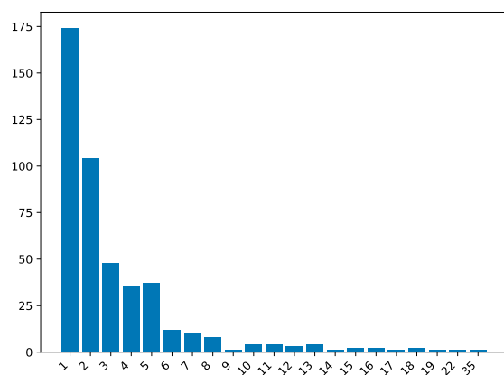
(a) SemEval2007
