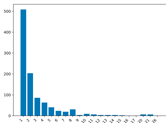
(c) SemEval2015
