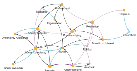
Figure 5: Causal graph directly generated by Gemma-2B-IT, Llama3-8B-IT, ValueBench upper-dimensions and human.
