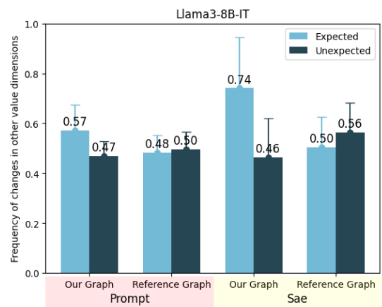
Figure 8: Comparing our casual graph and the causal graph generated from real-world human experiments.
