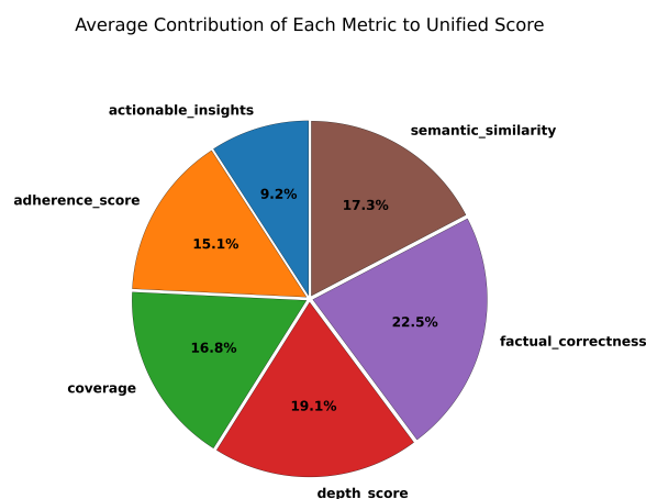
Figure 3: Metric Contribution
