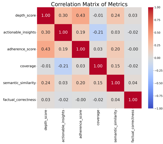
Figure 5: Correlation Heatmap
