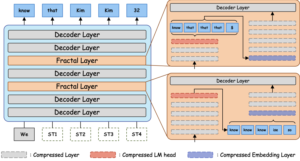
Figure 2: A schematic illustration of speculative decoding with proposed Fractal-LLM approach. The original hidden state passes through the compressed layers, produces provisional logits for draft tokens, re-embeds newly selected tokens, and merges them back into the main sequence.
