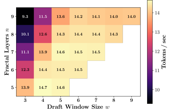
Figure 3: Inference acceleration (tokens/s) as a function of number of layers ( n ) and the draft window size ( w ).
