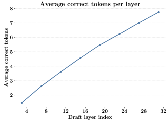
Figure 4: Average correct tokens per layer.
