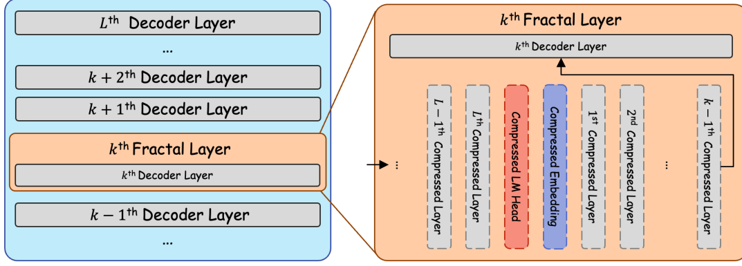
Figure 1: Structure of a Fractal Layer , where compressed modules (embedding, decoder layers, and LM head) are inserted before the i -th decoder layer to enable mid-forward draft token generation.
