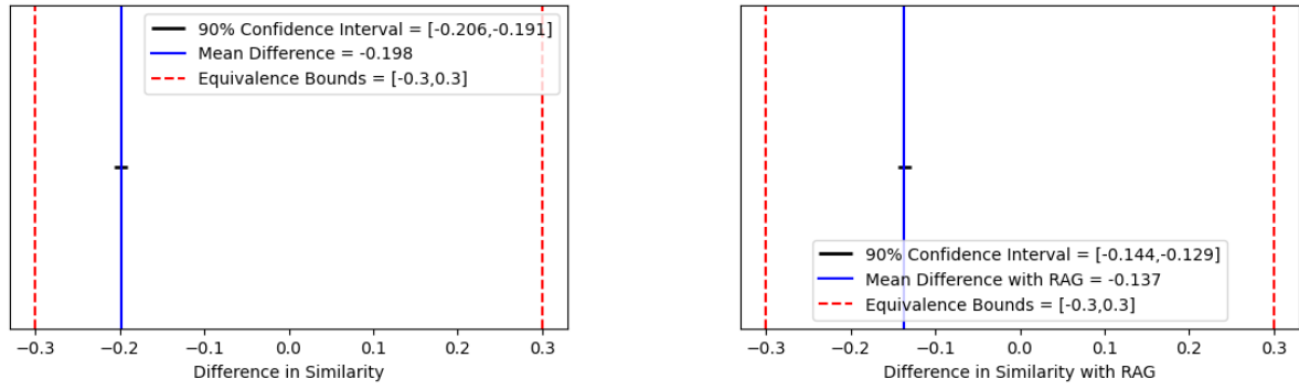
Figure 2: TOST between cosine similarities and Figure 3: TOST between cosine similarities and predicted similarities with RAG.
