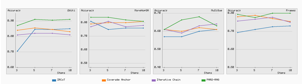
Figure 2: Step robustness results on answer quality, each panel compares IRCoT, Coverage Anchor, Iterative Chain, and PAR 2 -RAG across step counts 3, 5, 7, 10.
