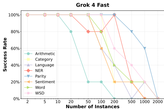
Figure 11: Success rate of models.
