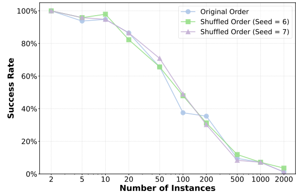
Figure 4: Success rates as a function of the number of instances for the original instance order and two shuffled variants constructed from the same instance sets.
