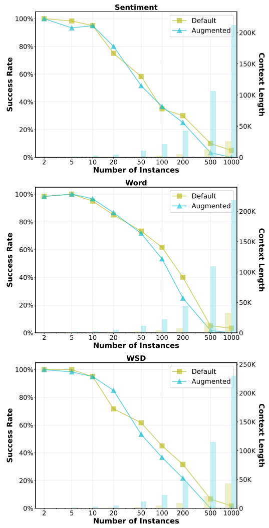
Figure 24: Success rate for tasks.
