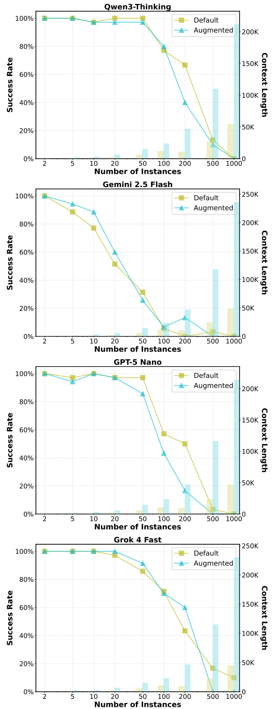
Figure 22: Success rate of models.
