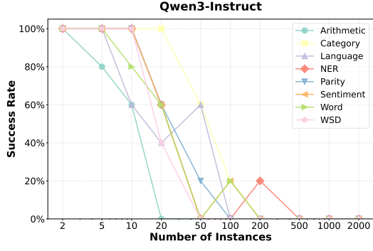
Figure 9: Success rate of models.
