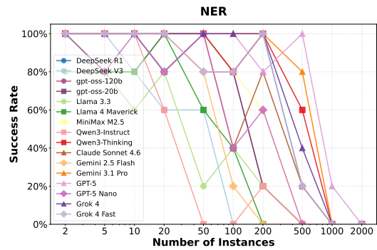
Figure 12: Model success rate for tasks.
