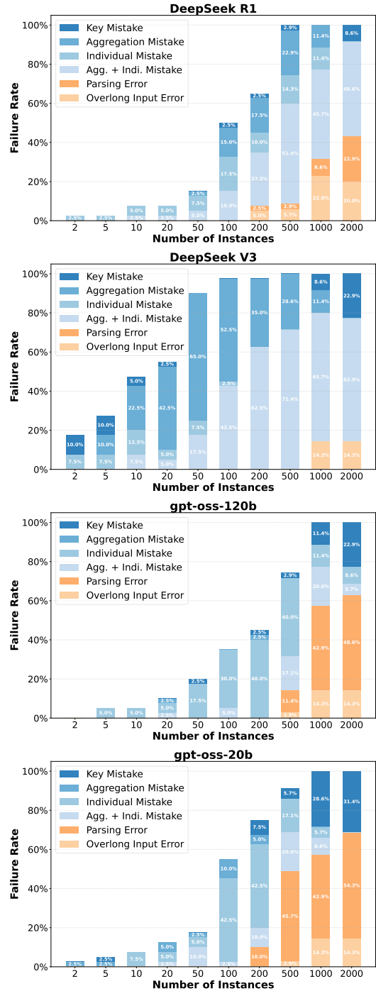
Figure 14: Failure rate breakdown for models.
