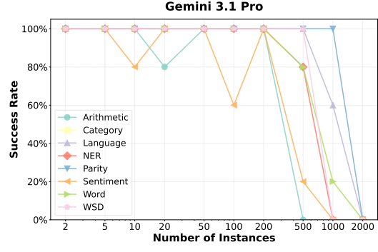
Figure 10: Success rate of models.
