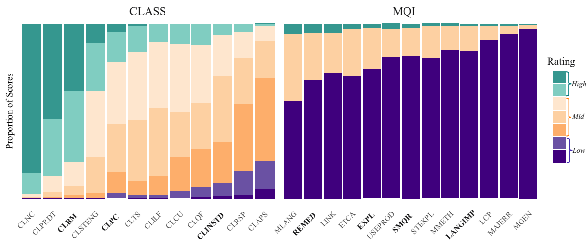
Figure 5: Proportions of human rater scores by item.
