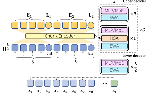
Figure 3: HSA-UltraLong model architecture.
