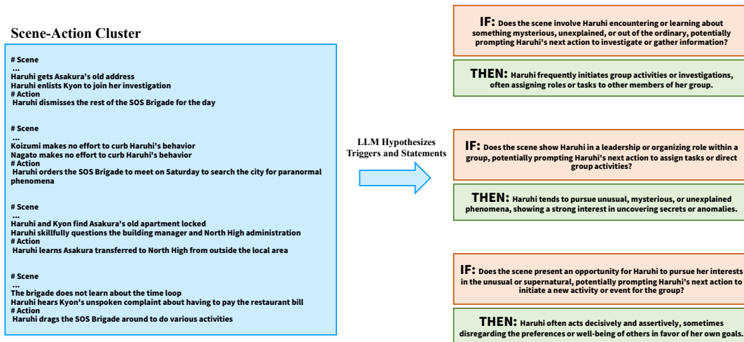
Figure 7: A running case for behavior hypothesis in the CDT building.
