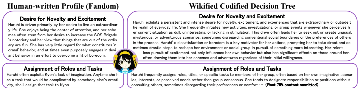
Figure 5: Granularity and coverage comparison between human profile and CDT. (Full wikified CDT in Figure 9, 10, and 11)
