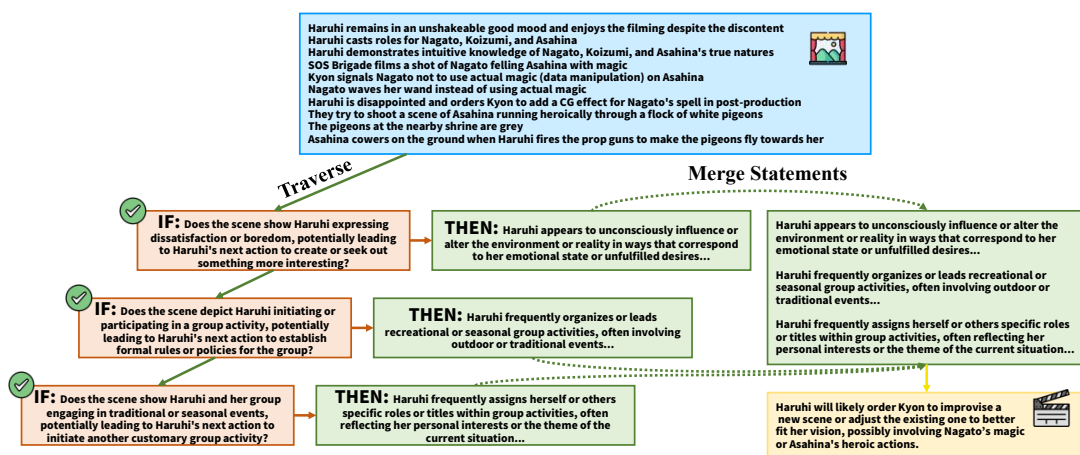
Figure 8: A running case for tree traversal in the CDT grounding.
