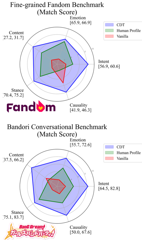
Figure 4: The comparison between grounding methods with matching scores. (CDT represents CDT-Lite)
