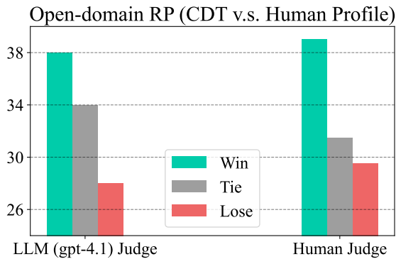
Figure 6: Comparison on open-ended RP by Human and LLM judgment. (CDT represents CDT-Lite)
