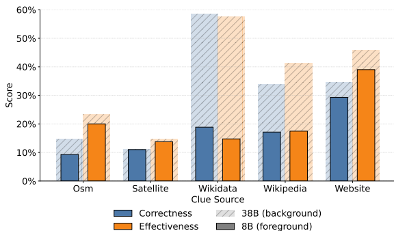
Figure 5: InternVL 3 (8B and 38B) correctness and effectiveness scores for each input. In these experiments, multi-turn pipeline with extended prompt and classification explanation is used.
