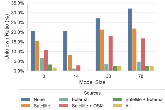
Figure 4: Baseline unknown ratio of InternVL 3 for input configurations. Unknown ratio corresponds to UNK ( uncertain ) responses over all inferences.
