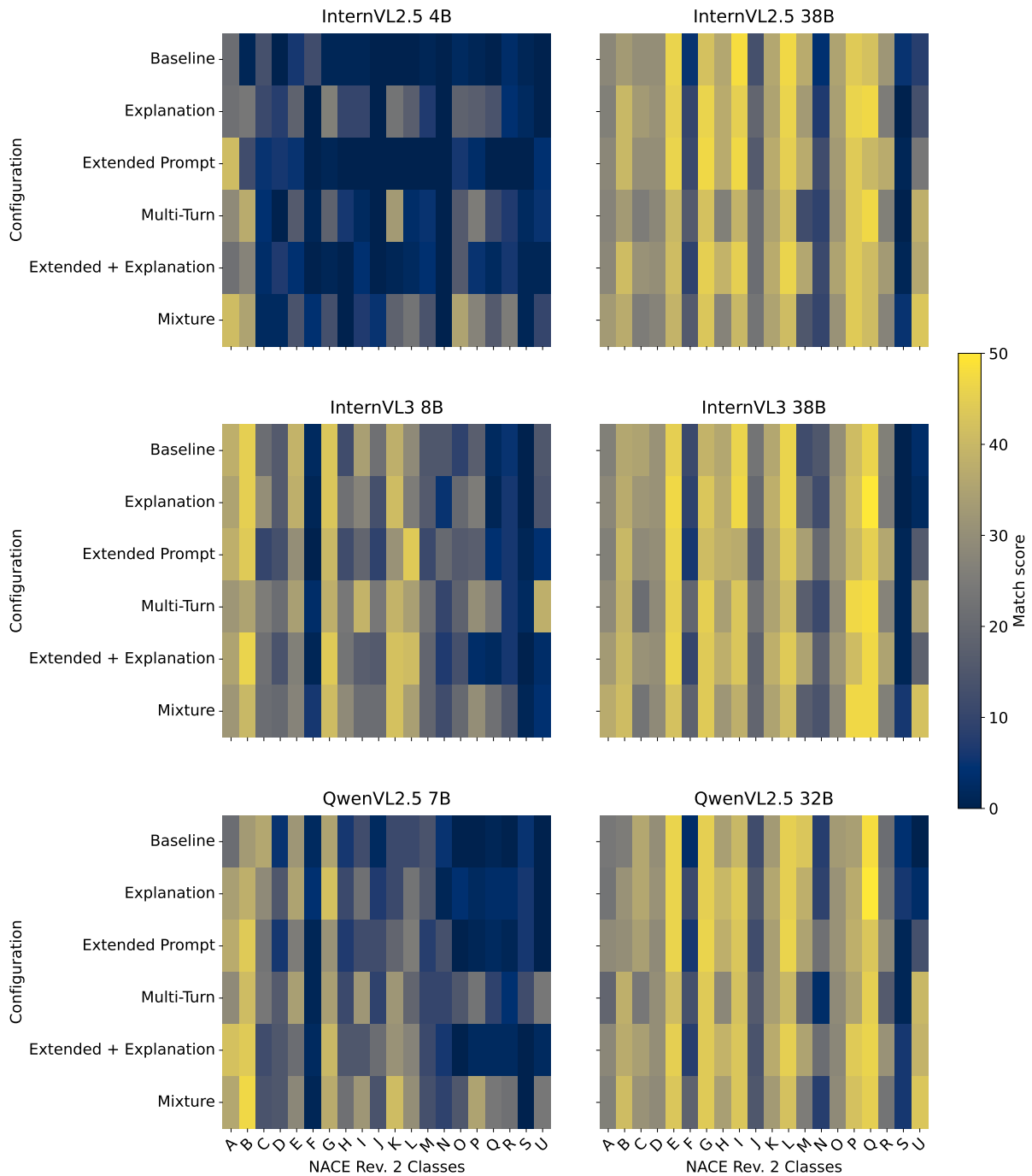
Figure 12: NACE Section-wise analysis for InternVL 2.5 (4B and 38B), InternVL 3 (8B and 38B), and QwenVL 2.5 (7B and 32B). Rows indicate experiment configurations. Mixture denotes Multi-Turn pipeline with classification explanations and prompt enrichment. Columns are the NACE section letters given in Table 8.
