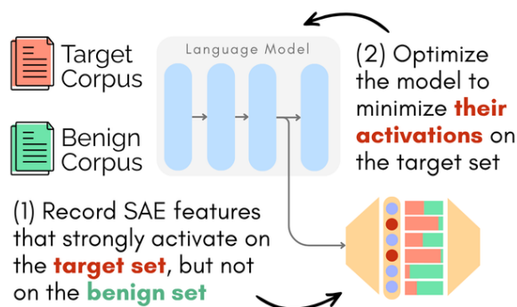
Figure 1: Overview of CRISP: (1) We identify features that are frequently and strongly activated by the target corpus—but not by the benign corpus—using pre-trained sparse autoencoders (SAEs). (2) We then fine-tune the model to suppress these features on the target corpus, while preserving their activations on the benign corpus.
