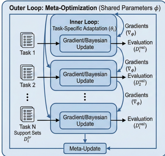
(a) Traditional Coupled Meta-Learning
