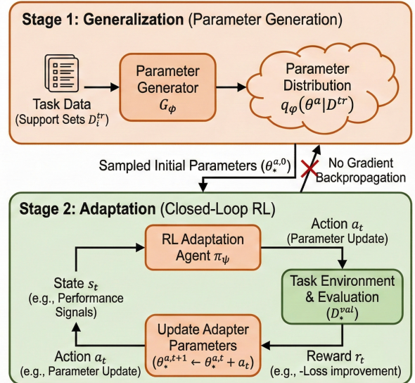
(b) Proposed DeGAML-LLM: Decoupled Generalization and Adaptation
