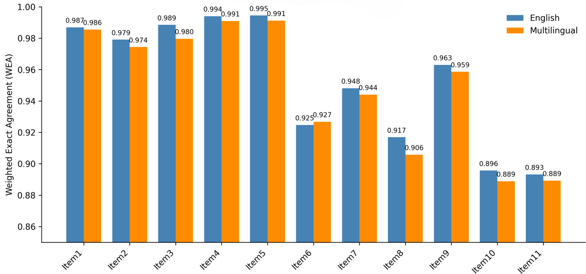
Figure 1: LiRA WEA by item, English vs. multilingual Qwen embeddings.
