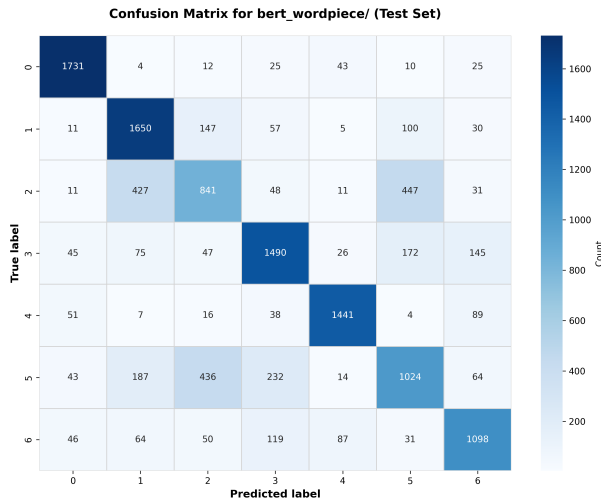
Figure 5: Confusion matrix for WordPiece
