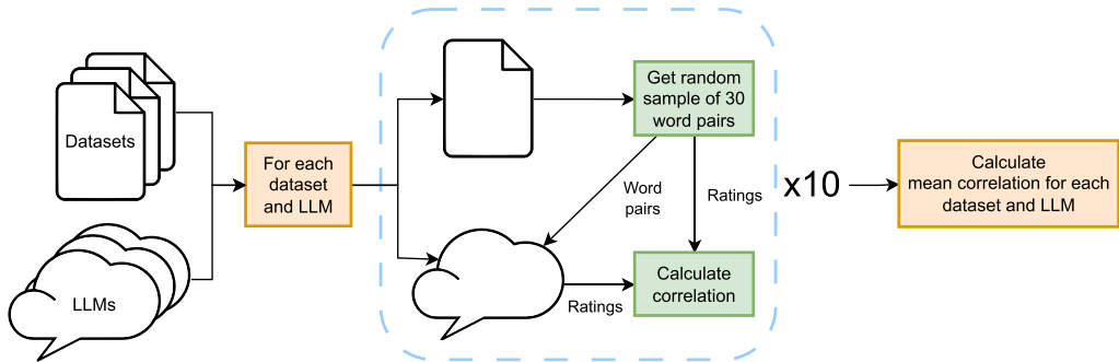
Figure 5 Pipeline for the evaluation of LLM ratings of SRs.
