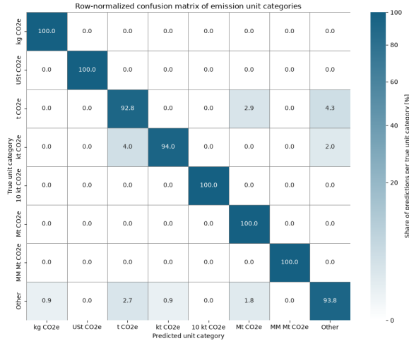
Figure 2: Confusion matrix of emission unit categories for the random-split dataset. Each row is normalized to 100%, showing the distribution of predicted unit categories for each true unit category. The diagonal entries correspond to the recall of the respective categories.
