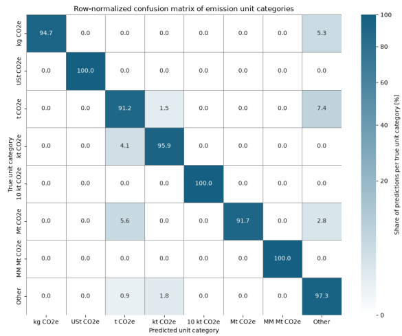
Figure A2: Row-normalized confusion matrix of predicted emission-unit categories on the rare-unit dataset. Values are percentages per true category; diagonal entries correspond to category-wise recall.
