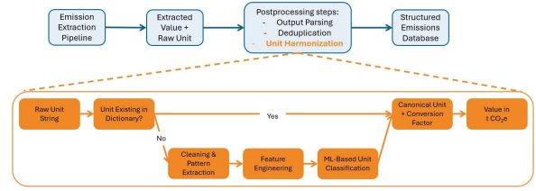
Figure 1: Overview of an emission extraction pipeline and the proposed hybrid extension for unit harmonization. In the evaluated extension, unresolved raw unit strings are passed to a machine learning fallback classifier before the extracted values are converted to t CO 2 e and stored in a structured emissions database.
