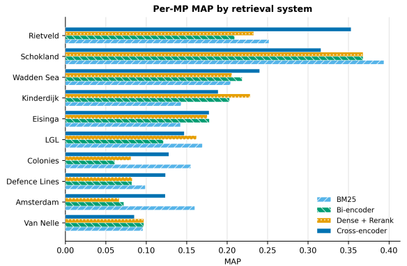
Figure 2: Per-MP MAP for all systems. MPs are sorted by the scores on Cross-encoder MAP.
