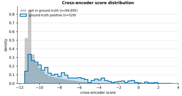
Figure 4: Cross-encoder score distribution for ground-truth positive chunks (GT) and all other chunks, aggregated across 24 labels. Distributions overlap because genuinely relevant but unannotated chunks score similarly to annotated positives.
