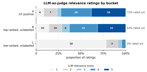
Figure 5: LLM relevance ratings by sampling bucket, shown as the proportion of ratings at each of the five discrete score levels (counts printed inside the bars, n = 140 ). Bucket B (top-ranked, unlabelled) is rated at least 4 almost as often as Bucket A (ground-truth positives), 62.9% vs. 72.3%, while Bucket C (low-ranked) is rated at least 4 only 4.3% of the time.
