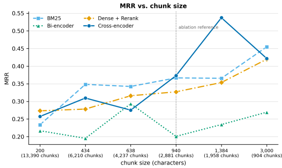
Figure 3: MRR computed over changing chunk sizes for all systems. The dotted line marks the 940-character grid point, the ablation’s closest configuration to the 1,000-character setting used for all primary results. Chunk counts are given under each grid point, since chunk size and corpus granularity vary together.
