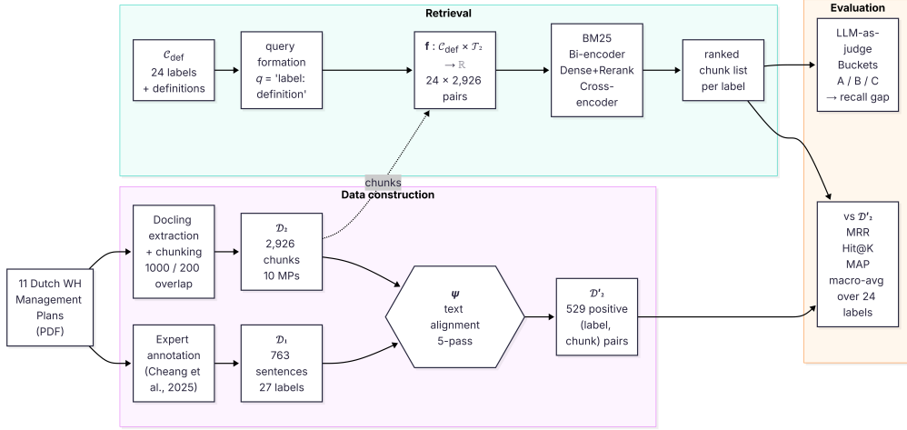
Figure 1: Overview of the pipeline. The same 11 Management Plans give rise to two datasets: the expert-annotated sentences \mathcal{D}_1 and the Docling-extracted chunks \mathcal{D}_2 . The alignment \psi links them into the chunk-level ground truth \mathcal{D}'_2 . Each concept in \mathcal{C}_{\text{def}} is turned into a query, the retrieval function f scores every label-chunk pair, and the resulting ranking is evaluated both against \mathcal{D}'_2 and by an LLM judge.
