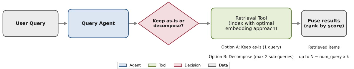
Figure 3: Query Agent Only workflow. The user query is rewritten and optionally decomposed into at most two sub-queries, each sent to the retrieval tool; the returned lists are fused and ranked by score.
