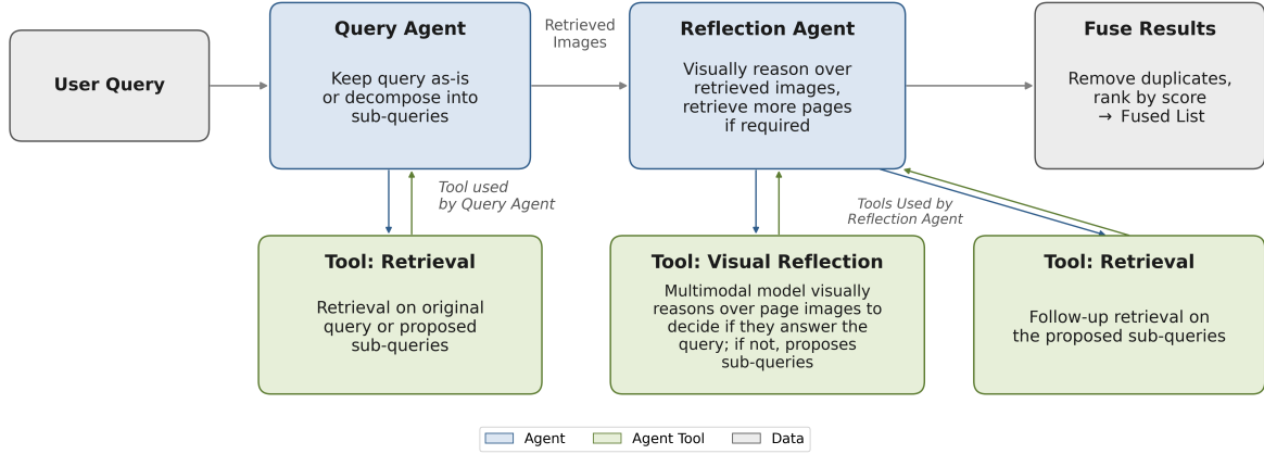
Figure 1: Reflect and Retrieve workflow centered on Reflection Agent. The Query Agent first keeps the user query as-is or decomposes it and retrieves an initial set of page images, which are sent to the Reflection Agent. The reflection agent calls a visual reflection tool, which uses a multimodal model to visually reason over the page images to decide whether they answer the query and, if not, proposes sub-queries; a retrieval tool then issues follow-up retrievals on those sub-queries. All retrieved items are fused by removing duplicates and ranking by score into the final fused list.
