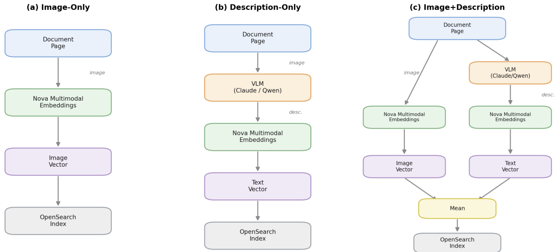
Figure 2: Three embedding strategies for page-level document indexing. (a) Image-Only embeds the raw page image directly. (b) Desc.-Only first generates a textual description with a VLM, then embeds the text. (c) Image+Desc. embeds the image and the description separately through Amazon Nova Multimodal Embeddings, then averages the two vectors.
