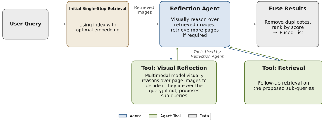
Figure 4: Reflection Agent Only workflow. An initial single-step retrieval, using the index with the optimal embedding, returns page images that are sent to the Reflection Agent. The agent calls a visual reflection tool, which uses a multimodal model to visually reason over the page images to decide whether they answer the query and, if not, proposes sub-queries; a retrieval tool then issues follow-up retrievals on those sub-queries. All retrieved items are fused by removing duplicates and ranking by score into the final fused list.
