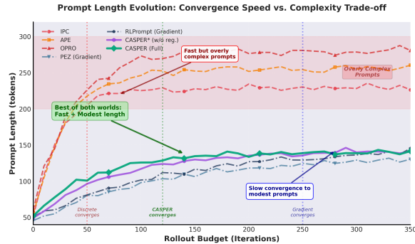
Figure 2: Prompt length evolution demonstrating CASPER’s efficiency-quality trade-off. Discrete methods (dashed) rapidly converge to complex prompts (220-280 tokens, <50 iterations), while gradient methods (dash-dot) slowly reach 140 tokens in 250 iterations. CASPER achieves comparable quality in 120 iterations—52% fewer than continuous optimization.
