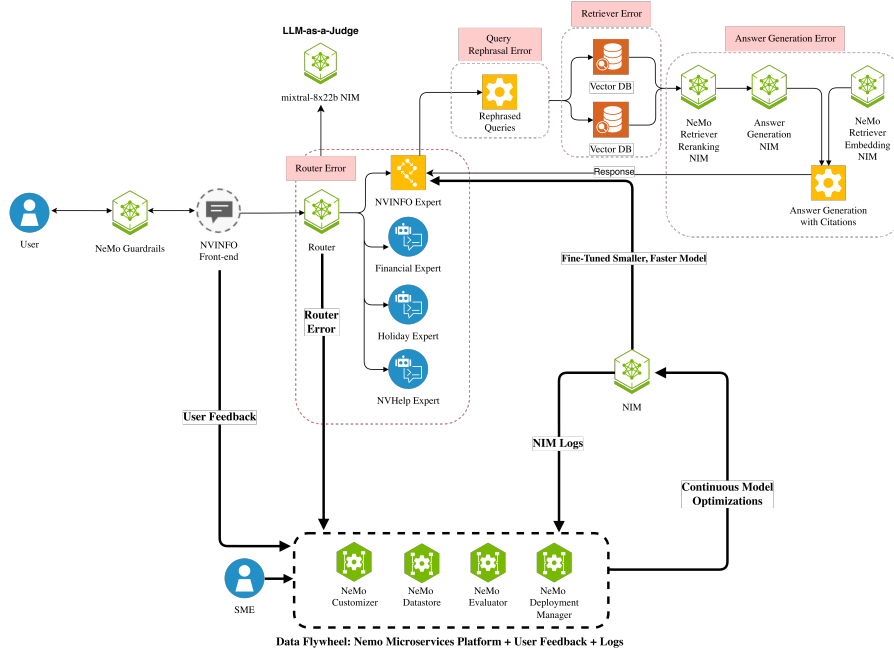
Figure 1: Adaptive Data Flywheel Architecture showing the MAPE control loop implementation for AI agent improvement
