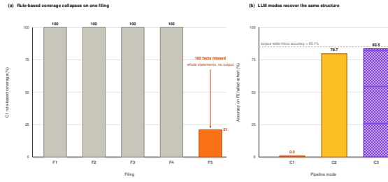
Figure 2: Catastrophic rule failure on F5. (a) C1 produces no output for 162 facts across whole sections, while coverage is complete on F1–F4. (b) On that cohort C1 scores 0%; C2 and C3 recover to 79.7% and 83.5% (dashed = corpus micro accuracy).
