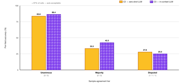
Figure 3: Per-field accuracy by sample-agreement tier (C2, C3). Accuracy falls from unanimous to disputed, so agreement ranks predictions by reliability; we use it as a triage signal for targeted review, not a guarantee.
