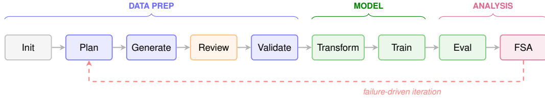
Figure 3: Data pipeline across three phases. Blue = LLM agents. Green = deterministic code. Orange = human approval. Dashed loop: FSA drives next iteration’s planning.
