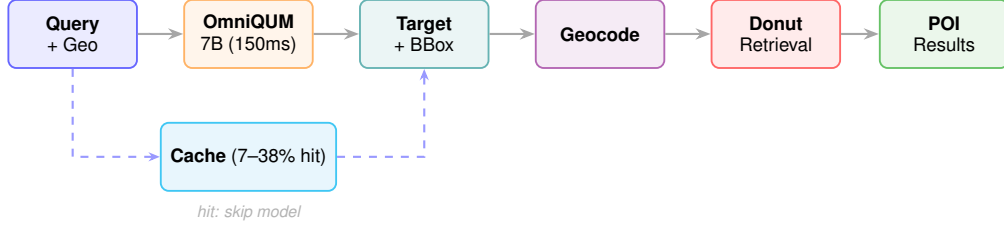
Figure 2: End-to-end architecture. On cache miss, OmniQUM produces a disambiguated target and bounding box; the target is geocoded, then donut retrieval finds POIs from successive distance rings.
