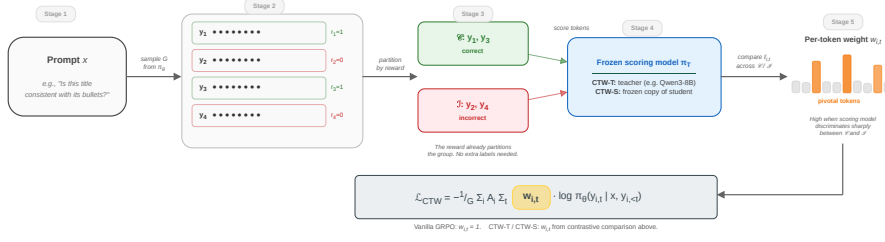
Figure 1: CTW pipeline. The reward partitions a GRPO group into correct ( \mathcal{C} ) and incorrect ( \mathcal{I} ); a frozen scorer (CTW-T: teacher, CTW-S: student copy) scores tokens across both subsets, and divergent positions receive higher w_{i,t} in the policy loss.
