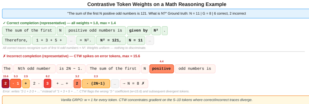
Figure 3: CTW-T weights on a MATH problem (Qwen3-1.7B student, 8B teacher). Both subsets receive a contrastive signal (Eq. 3); the weights concentrate on a few tokens where the scorer most sharply separates correct from incorrect completions, while most positions stay near the uniform weight of 1.
