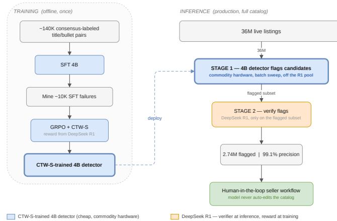
Figure 2: Production cascade. Training (left) : consensus labels train a 4B SFT detector, refined by GRPO + CTW-S on its failures with DeepSeek R1 as reward. Inference (right) : the deployed 4B detector (blue) flags all 36M listings; R1 (orange) verifies only the flagged subset, reaching 99.1% cascade precision before human review.
