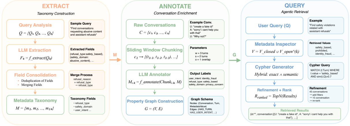
Figure 1: Extract-Annotate-Query Framework for Conversational Data Retrieval
