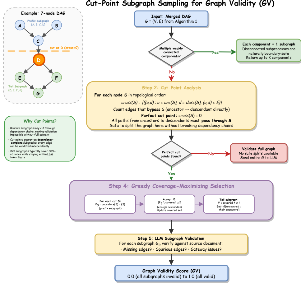
Figure 4: Cut-point subgraph sampling for Graph Validity: the DAG is split at nodes with zero cross-edges into boundary-safe subgraphs for independent LLM validation.
