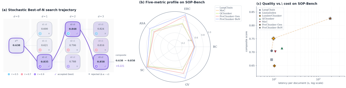
Figure 2: (a) Stochastic Best-of-N trajectory on SOP-Bench/warehouse_package_inspection: three candidates fan out at \tau \in \{0.5, 0.7, 0.9\} per depth, \epsilon -gate accepts the best ( \checkmark ) and rejects the rest ( \times ). (b) Five-metric profile on SOP-Bench: ProChunker-BoN dominates on ERC and GV while baselines saturate SC. (c) Quality vs. latency on SOP-Bench: ProChunker-Gen and -BoN sit on the Pareto frontier (dashed line)
