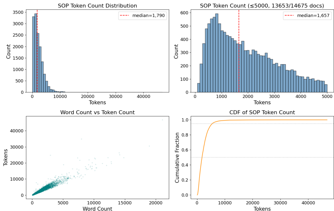
Figure 3: Token length distribution of BioProbench SOPs. The distribution is heavily right-skewed with a median of 1,790 tokens.
