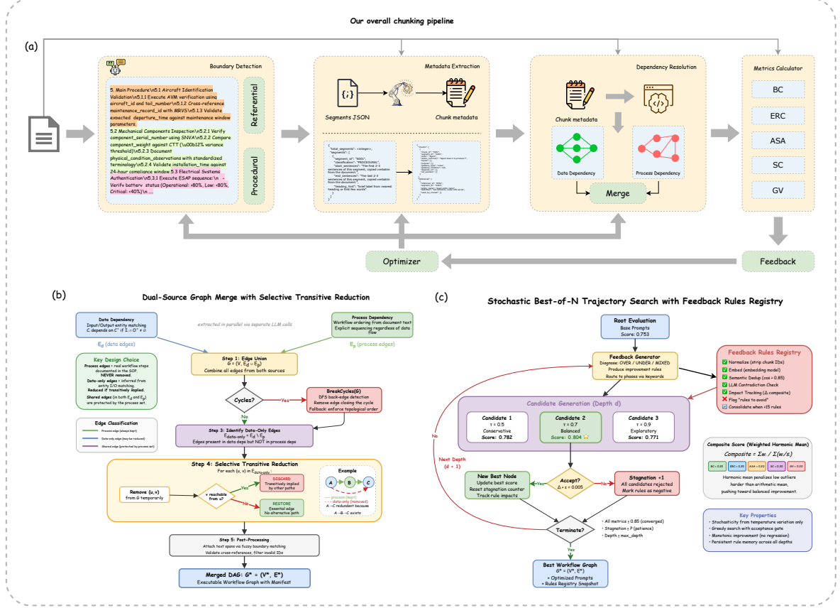
Figure 1: Overview of the proposed framework. (a) Three-phase chunking pipeline with five evaluation metrics and a closed-loop prompt optimization cycle. (b) Dual-source graph merge: data and process edges are unioned, cycles broken via DFS, and selective transitive reduction removes only data-only edges implied by alternative paths; process edges are never removed. (c) Stochastic Best-of-N search: three candidates at varied temperatures are evaluated per depth, accepted only on improvement, with a persistent rules registry preventing regression.
