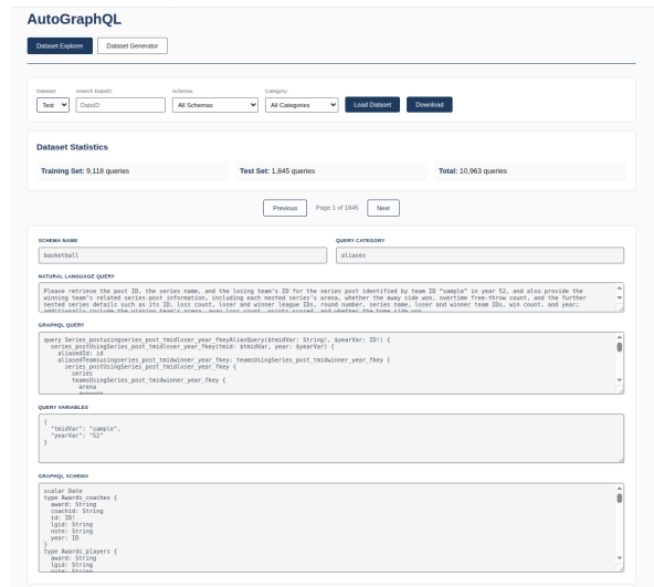
(b) Dataset Exploration Interface
