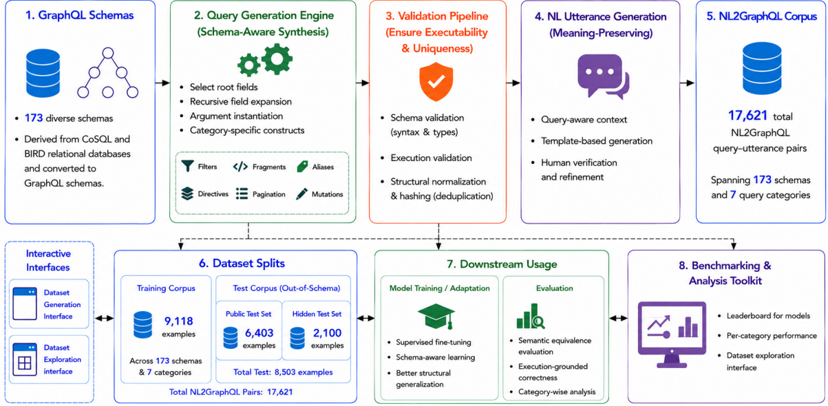
Figure 2: Overview of the proposed AutoGraphQL framework.
