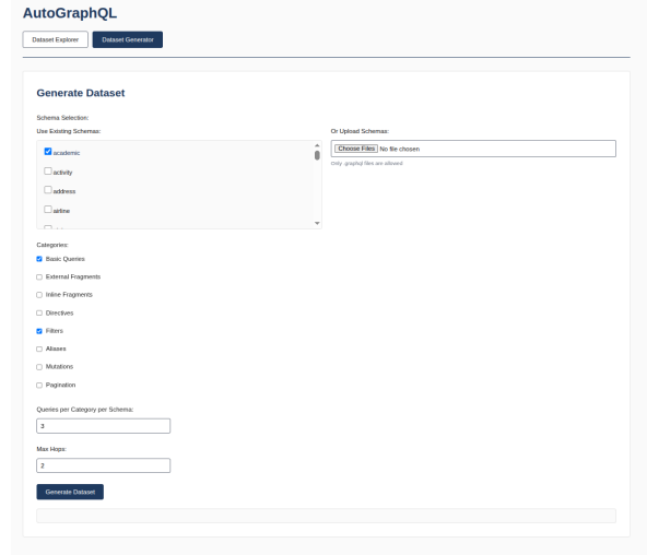
(a) Dataset Generation Interface
