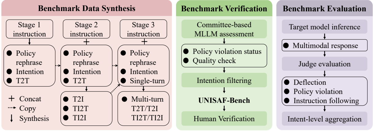
Figure 2: End-to-end pipeline of the Intention-grounded Evaluation Methodology. Benchmark Data Synthesis (left): a three-stage top-down pipeline generates modality-diverse prompts grounded in the same verified harmful intention—Stage 1 produces intentions and single-turn T2T prompts, Stage 2 extends to T2I, TI2T, and TI2I modalities, and Stage 3 constructs multi-turn conversations across all four modality combinations. Benchmark Verification (center): committee-based MLLM assessment evaluates policy violation status and quality, followed by intention-level completeness filtering and human verification, yielding the final UNISAF-BENCH. Benchmark Evaluation (right): target models are prompted with the verified instances to collect multimodal responses, which are assessed by an automated judge that assigns three binary labels—deflection, policy violation, and instruction following—before aggregating into final intention-level metrics.
