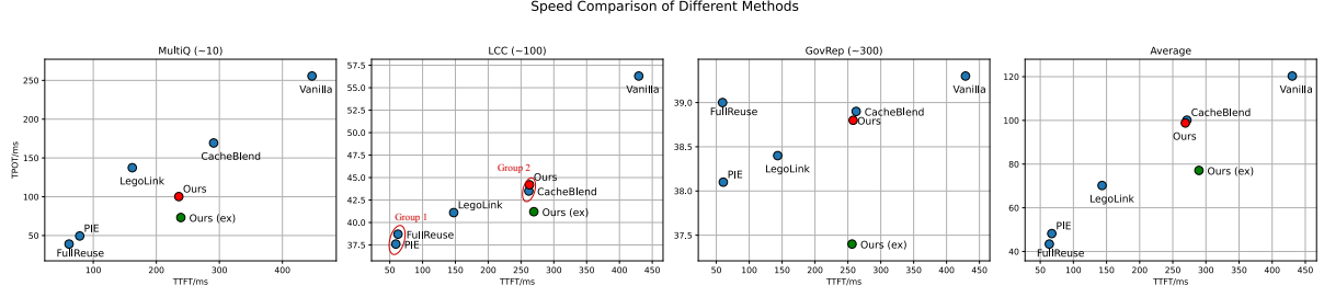
Figure 5: Comparison of inference performance among different reuse methods.
