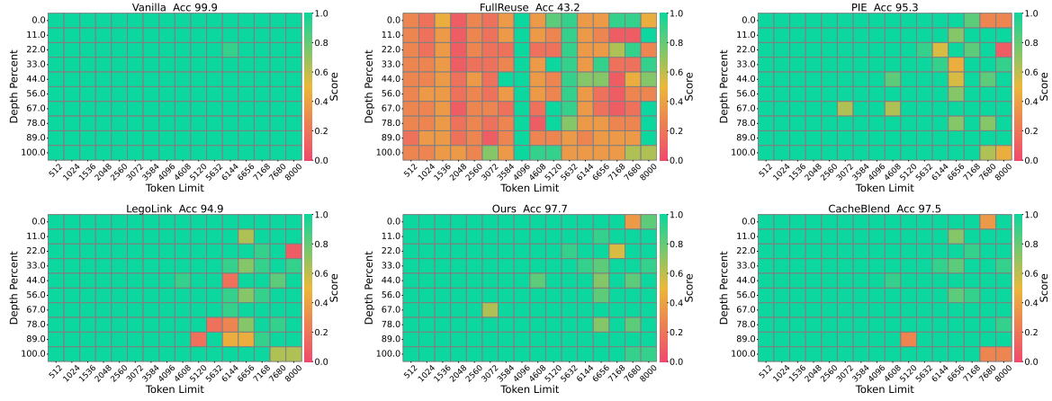
Figure 7: Needle-in-a-Haystack results on Qwen2.5-7B-Instruct and Mistral-7B-Instruct-v0.2. The vertical axis represents depth percentage, and the horizontal axis represents token length. Our method achieves the best retrieval performance.
