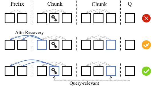
Figure 1: Blue blocks indicate that the corresponding KVs are recomputed. (Top) Without recomputation. (Middle) Recomputation applied but key information missed. (Bottom) Key information updated based on query-aware attention.
