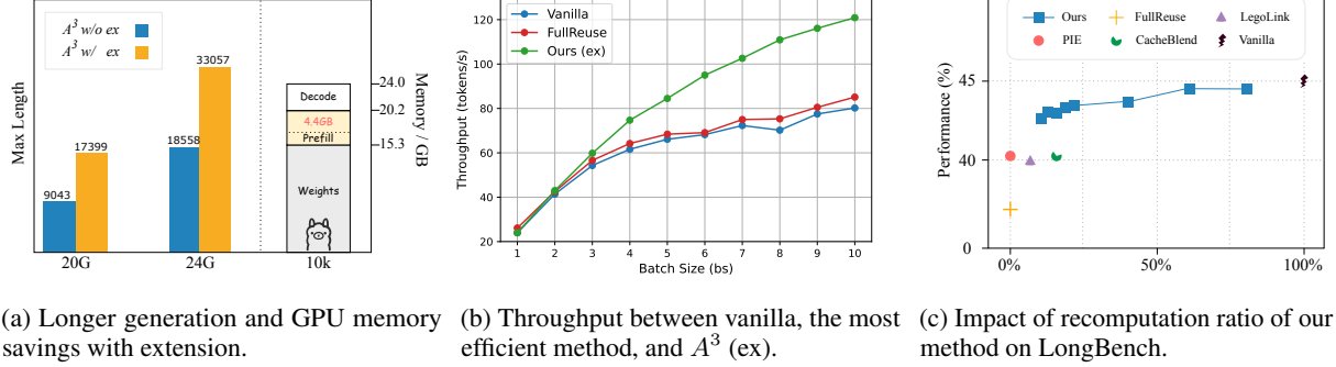
Figure 6: Inference performance analysis of A^3 , illustrating latency variations with the acceleration extension and ablation studies on key hyperparameters.
