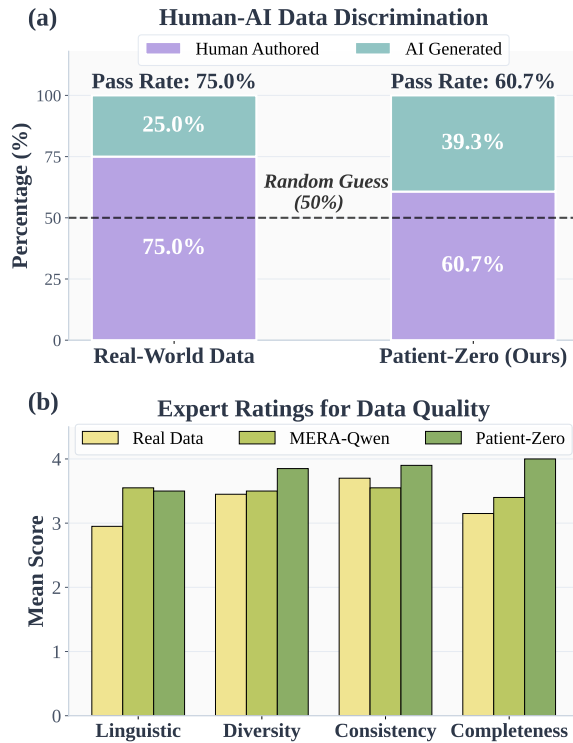
Figure 5: Expert Evaluation Results. (a) Senior licensed physicians judge discrimination between real and synthetic records. (b) Patient-Zero obtained the highest diversity, consistency, and completeness means.
