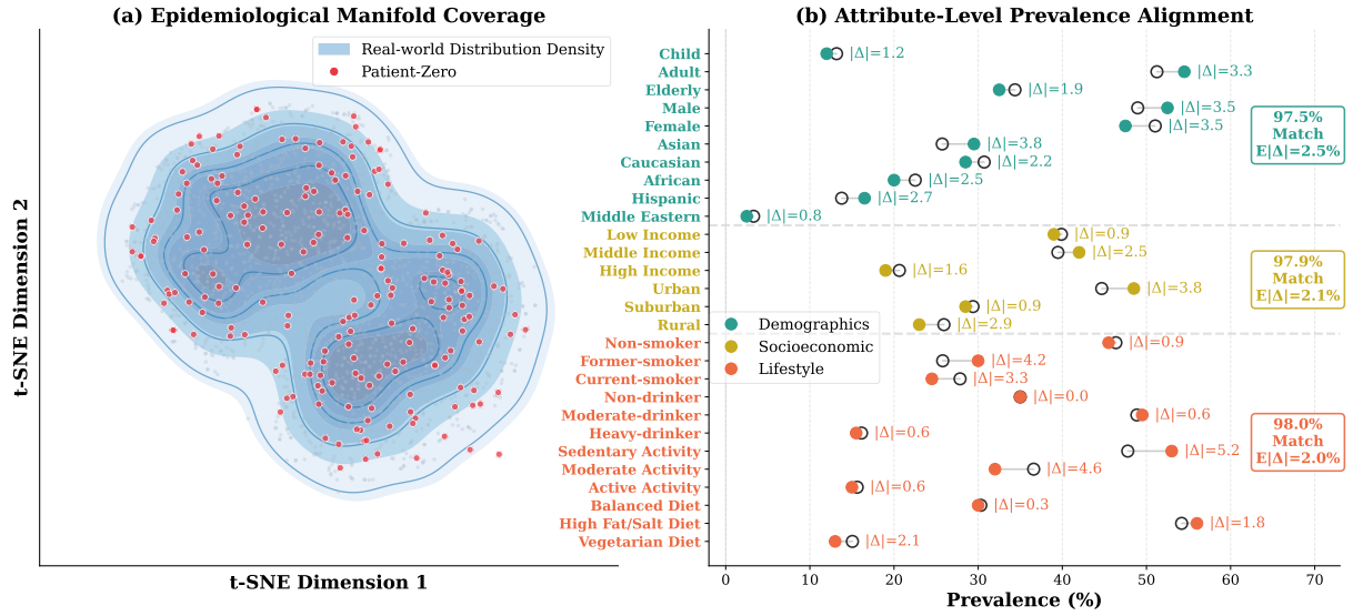
Figure 4: Holistic Epidemiological and Semantic Alignment. (a) Epidemiological Manifold Coverage: The tight overlap of t-SNE visualization in the high-dimensional semantic space indicates that our synthetic data captures the comprehensive epidemiological manifold without mode collapse. (b) Attribute-Level Prevalence Alignment: Prevalence comparison across three dimensions. Hollow circles (○) represent real-world baseline; solid circles (●) represent Patient-Zero ; the connecting lines indicate alignment gaps. Minimal absolute differences demonstrate that Patient-Zero faithfully reconstructs complex real-world demographic and behavioral profiles.
