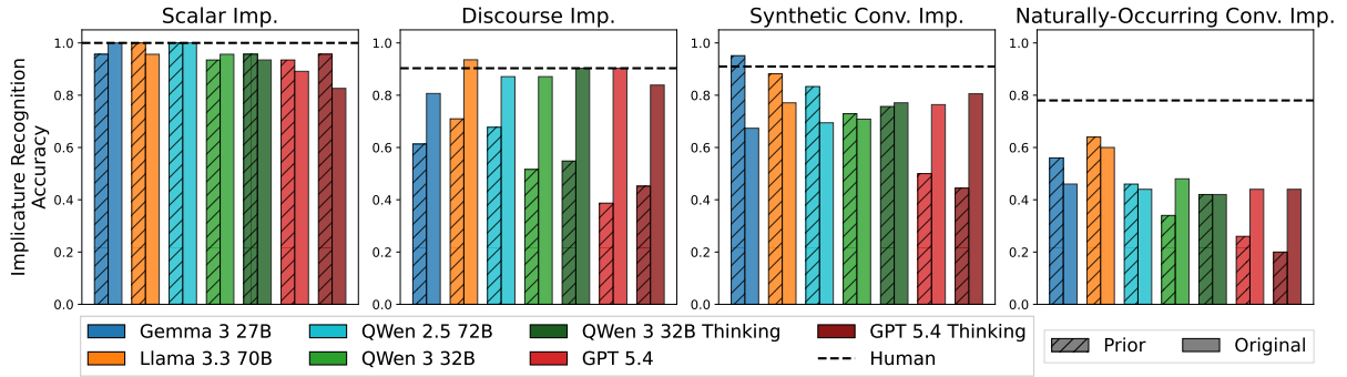
Figure 4: Implicature recognition accuracies of the largest and most modern models for each class of models tested. Original denotes the accuracy using the t_b(c, u) prompt and prior denotes the accuracy using the t_b(\emptyset, \emptyset) prompt.
