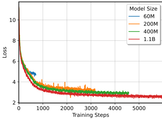
Figure 7: Pre-training loss of CLM series.
