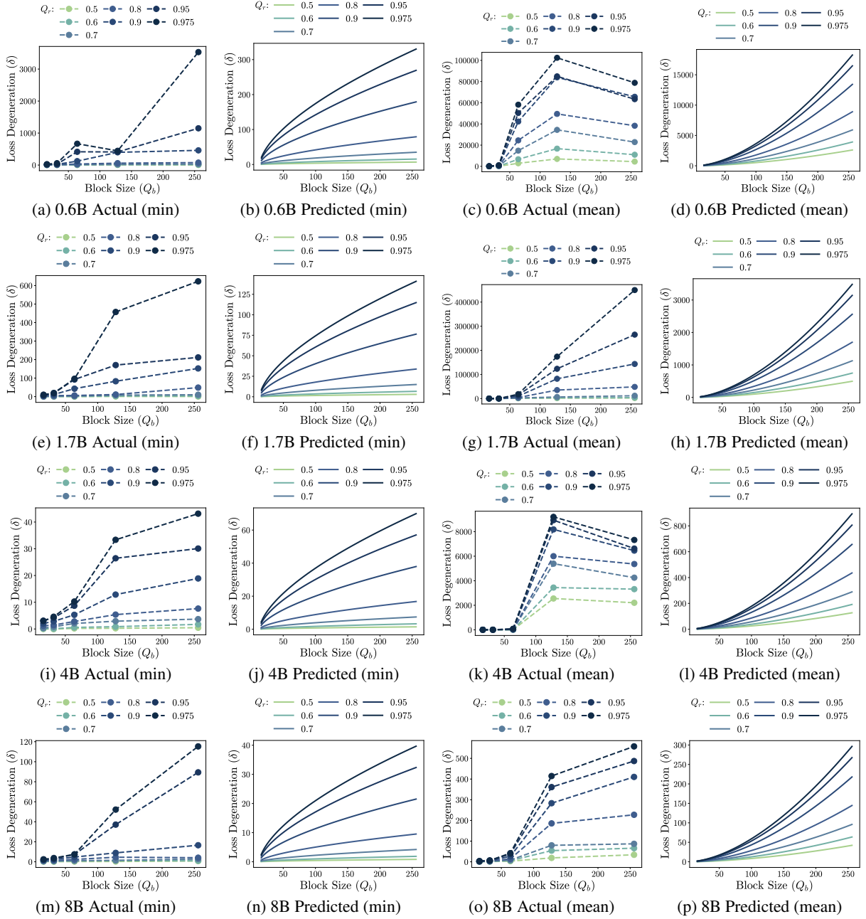
Figure 15: Strong Law Qwen-3 Matrix Multiplication-wise ( \delta^{\text{opt}} , \delta_\mu ) (a,b,e,f,i,j,m,n) Qwen-3 matrix multiplication-wise \delta^{\text{opt}} results; (c,d,g,h,k,l,o,p) Qwen-3 matrix multiplication-wise \delta_\mu results.
