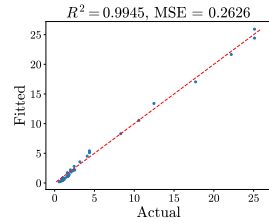
Figure 38: Minifloat Qwen-3 Weak Law. The left two are for \delta^{\text{opt}} and the right two are for \delta_\mu .
