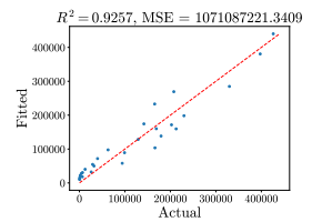
Figure 42: MXINT-2 CLM Weak Law. The left two are for \delta^{\text{opt}} and the right two are for \delta_\mu .
