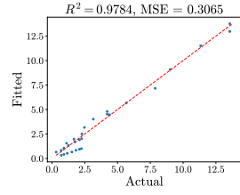
Figure 48: MXINT-4 Matrix Multiplication-wise Qwen-1.5 Weak Law. The left two are for \delta^{\text{opt}} and the right two are for \delta_\mu .
