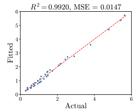
Figure 50: MXINT-4 Matrix Multiplication-wise Qwen-3 Weak Law. The left two are for \delta^{\text{opt}} and the right two are for \delta_\mu .
