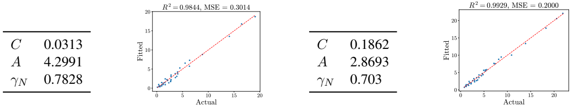
Figure 45: MXINT-4 Layerwise CLM Weak Law. The left two are for \delta^{\text{opt}} and the right two are for \delta_\mu .
