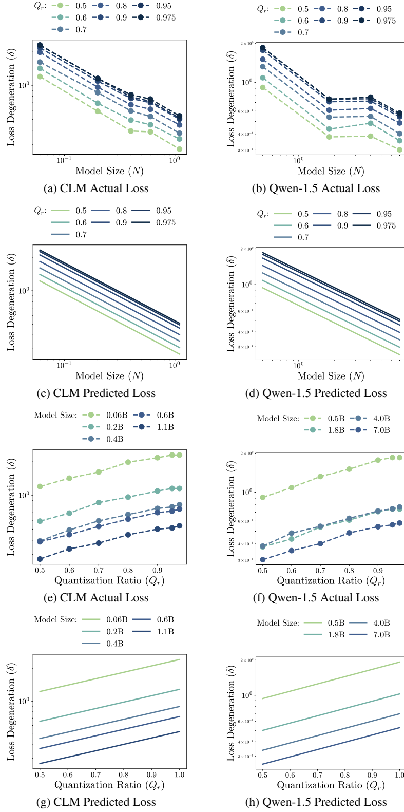
Figure 19: GPTQ ( \delta_\mu ) (a,c,e,g) CLM GPTQ results; (b,d,f,h) Qwen-1.5 GPTQ results.
