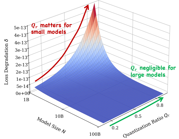
Figure 1: Visualization of mixed-precision scaling law. Loss degradation \delta decreases with model size N , but increases with quantization ratio Q_r . The fitted parameters are obtained from experiments on the Qwen-3 models with block size Q_b = 32 .
