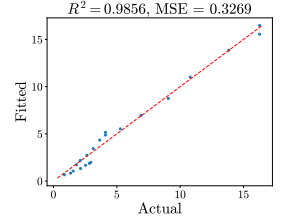
Figure 37: Minifloat Qwen-1.5 Weak Law. The left two are for \delta^{\text{opt}} and the right two are for \delta_\mu .
