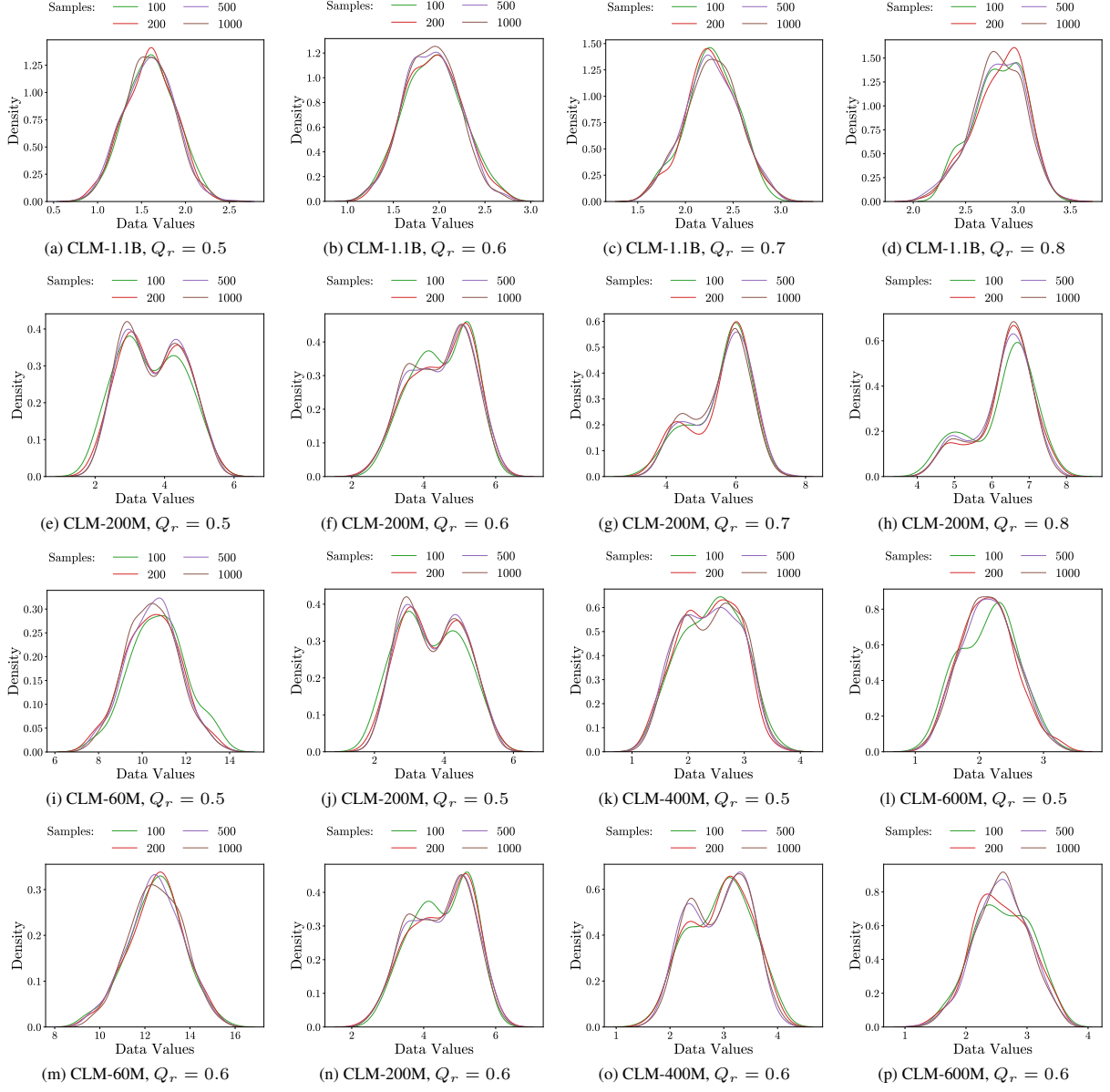
Figure 8: KDE of distribution \delta . Different KDE for different Q_r under a fixed model: (a,b,c,d) Changing Q_r for CLM-1.1B; (e,f,g,h) Changing Q_r for CLM-200M. KDE for different model under fixed Q_r ; (i,j,k,l) Changing N for Q_r = 0.5 ; (m,n,o,p) Changing N for Q_r = 0.6 .
