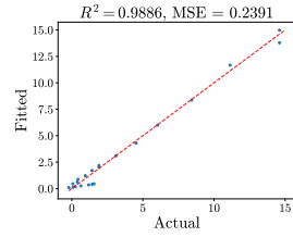
Figure 37: Minifloat Qwen-1.5 Weak Law. The left two are for \delta^{\text{opt}} and the right two are for \delta_\mu .
