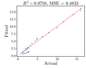
Figure 48: MXINT-4 Matrix Multiplication-wise Qwen-1.5 Weak Law. The left two are for \delta^{\text{opt}} and the right two are for \delta_\mu .
