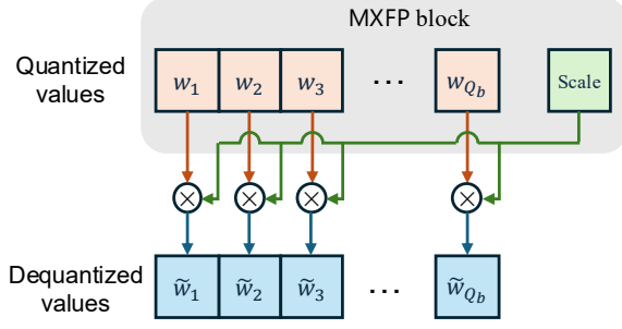
Figure 2: MXFP block with Q_b values sharing one scale. A larger block size Q_b shares one scale across more values, reducing scale overhead but typically increasing quantization error due to a coarser dynamic-range fit.
