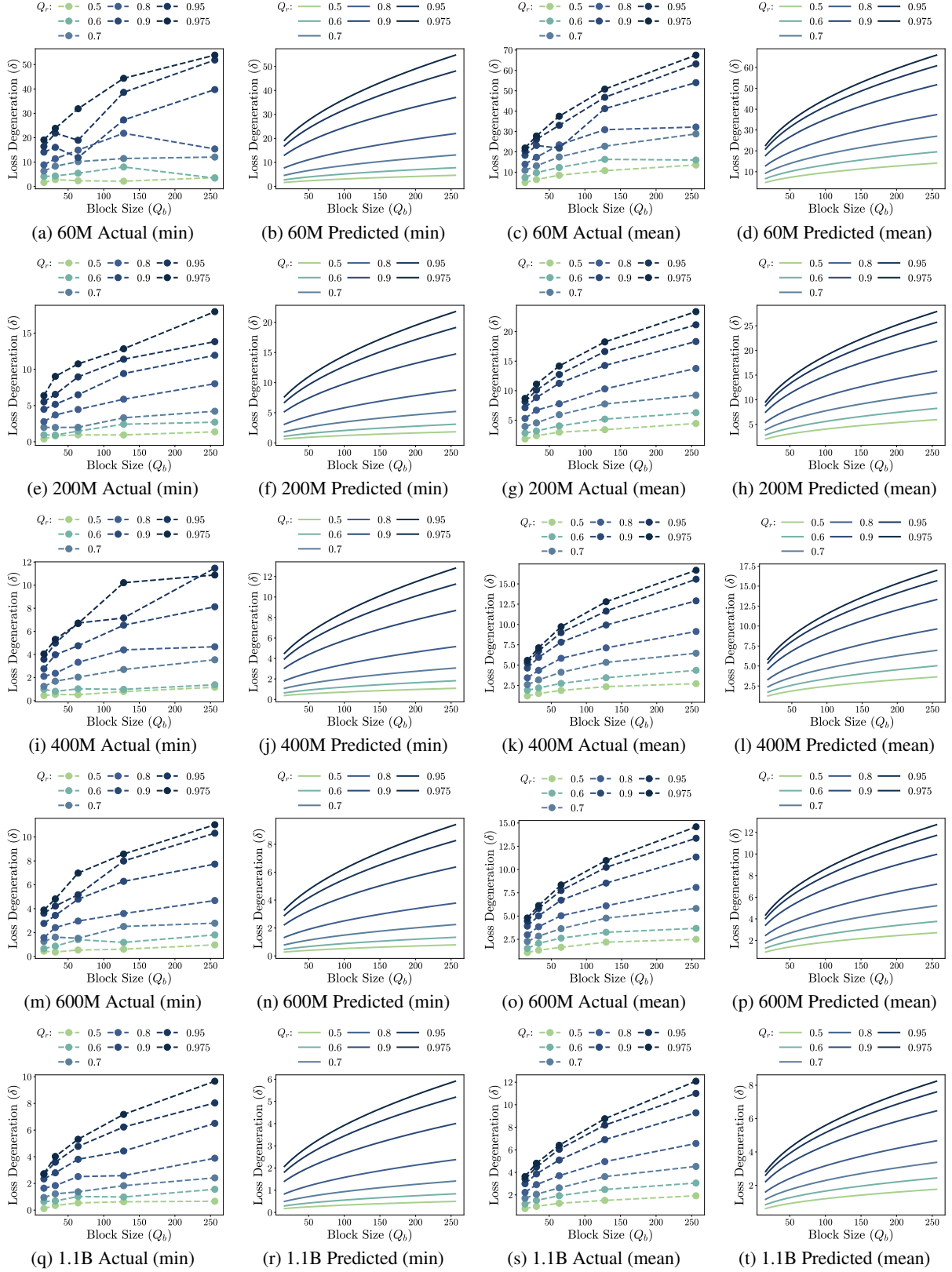
Figure 13: Strong Law CLM Matrix Multiplication-wise ( \delta^{\text{opt}} , \delta_\mu ) (a,b,e,f,i,j,m,n,q,r) CLM matrix multiplication-wise \delta^{\text{opt}} results; (c,d,g,h,k,l,o,p,s,t) CLM matrix multiplication-wise \delta_\mu results.
