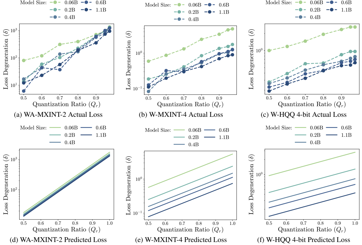
Figure 5: Other Arithmetic Formats Results. (a,d) The actual and fitted loss degradation contour for layer-wise Weight-Activation-MXINT-2 (WA-MXINT-2) on CLM architectures. (b,e) The actual and fitted loss degradation contour for layer-wise Weight-only MXINT-4 (W-MXINT-4) on CLM architectures. (c,f) The actual and fitted loss degradation contour for layer-wise Weight-only 4bit-HQQ (HQQ-4) on CLM architectures. In the figure, each line corresponds to a fixed model size N in billions (B). The fitted statistics are presented in Appendix F due to space constraints.
