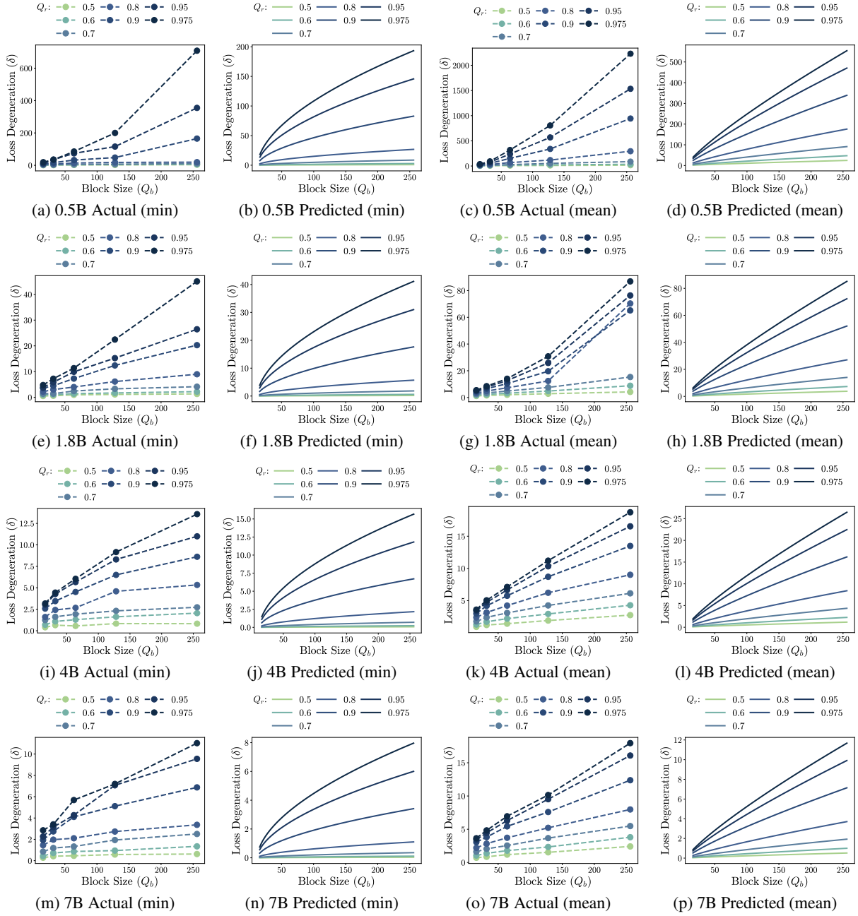
Figure 14: Strong Law Qwen-1.5 Matrix Multiplication-wise ( \delta^{\text{opt}} , \delta_\mu ) (a,b,e,f,i,j,m,n) Qwen1.5 matrix multiplication-wise \delta^{\text{opt}} results; (c,d,g,h,k,l,o,p) Qwen-1.5 matrix multiplication-wise \delta_\mu results.
