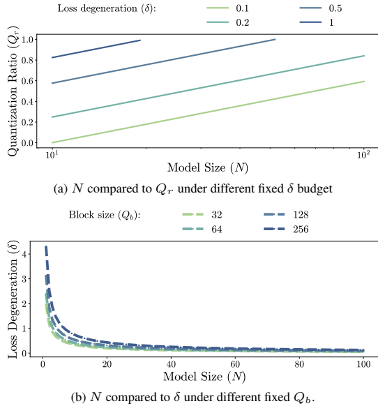
Figure 6: Effects of our scaling laws. The effect of our scaling law with (a) effect of quantization ratio Q_r when changing model size N under a fixed loss degradation budget \delta and (b) effect of block size granularities Q_b on loss degradation \delta when changing N . Both are based on the fitted parameters for CLM series models.
