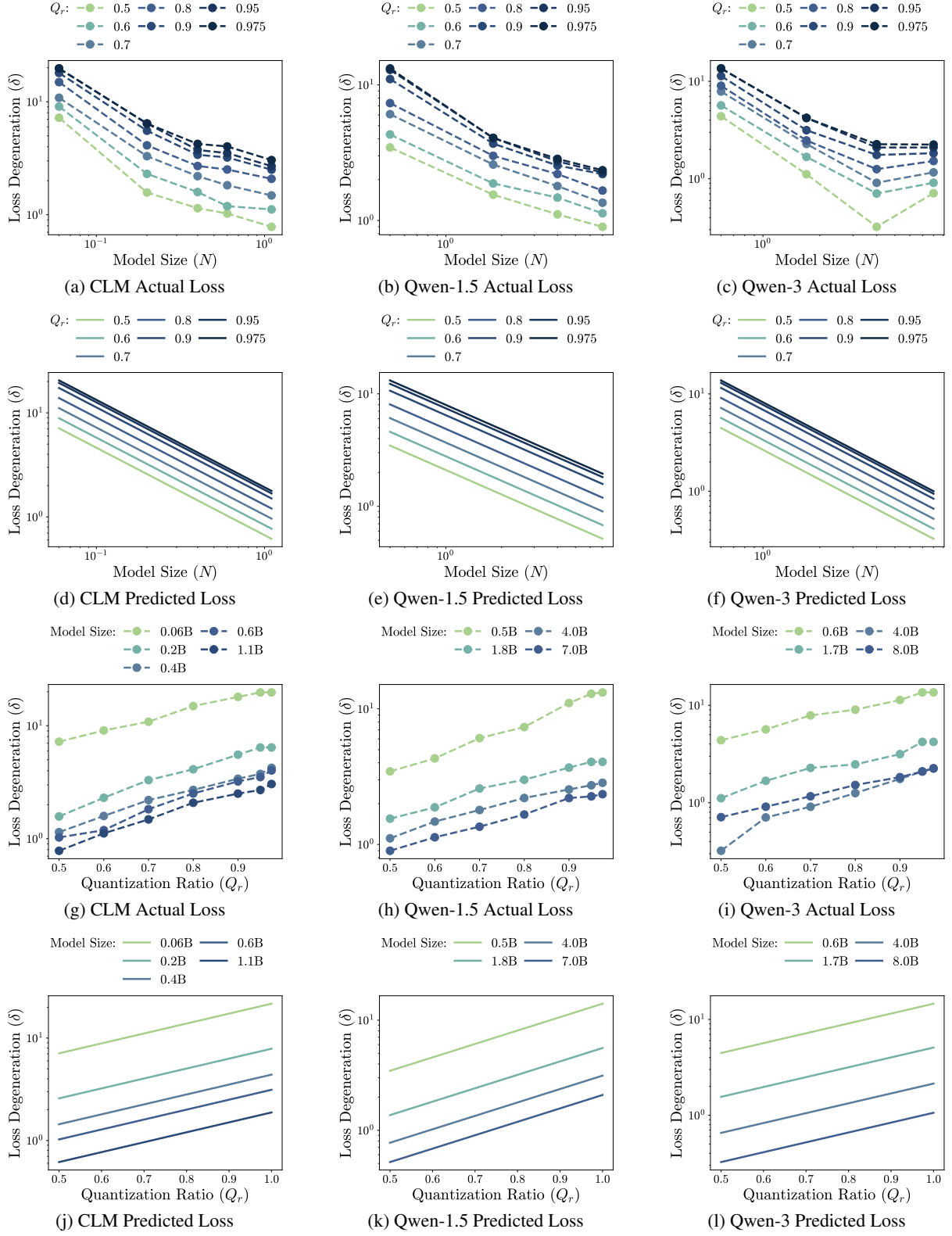
Figure 9: Layer-wise ( \delta^{\text{opt}} ) (a,d,g,h) CLM layer-wise results; (b,e,h,k) Qwen-1.5 layer-wise results; (c,f,i,l) Qwen-3 layer-wise results.
