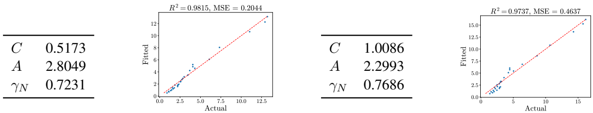
Figure 46: MXINT-4 Matrix Multiplication-wise CLM Weak Law. The left two are for \delta^{\text{opt}} and the right two are for \delta_\mu .
