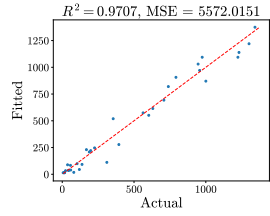
Figure 41: MXFP Qwen-3 Weak Law. The left two are for \delta^{\text{opt}} and the right two are for \delta_\mu .
