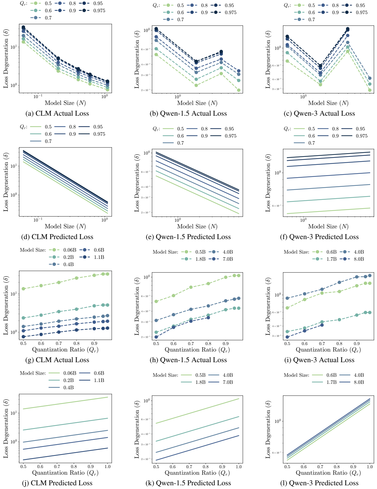
Figure 23: MXFP ( \delta_\mu ) (a,d,g,h) CLM MXFP results; (b,e,h,k) Qwen-1.5 MXFP results; (c,f,i,l) Qwen-3 MXFP results.
