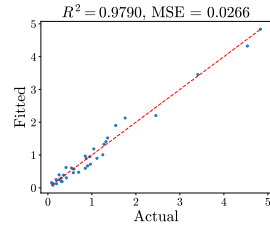
Figure 50: MXINT-4 Matrix Multiplication-wise Qwen-3 Weak Law. The left two are for \delta^{\text{opt}} and the right two are for \delta_\mu .
