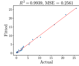
Figure 49: MXINT-4 Layerwise Qwen-3 Weak Law. The left two are for \delta^{\text{opt}} and the right two are for \delta_\mu .
