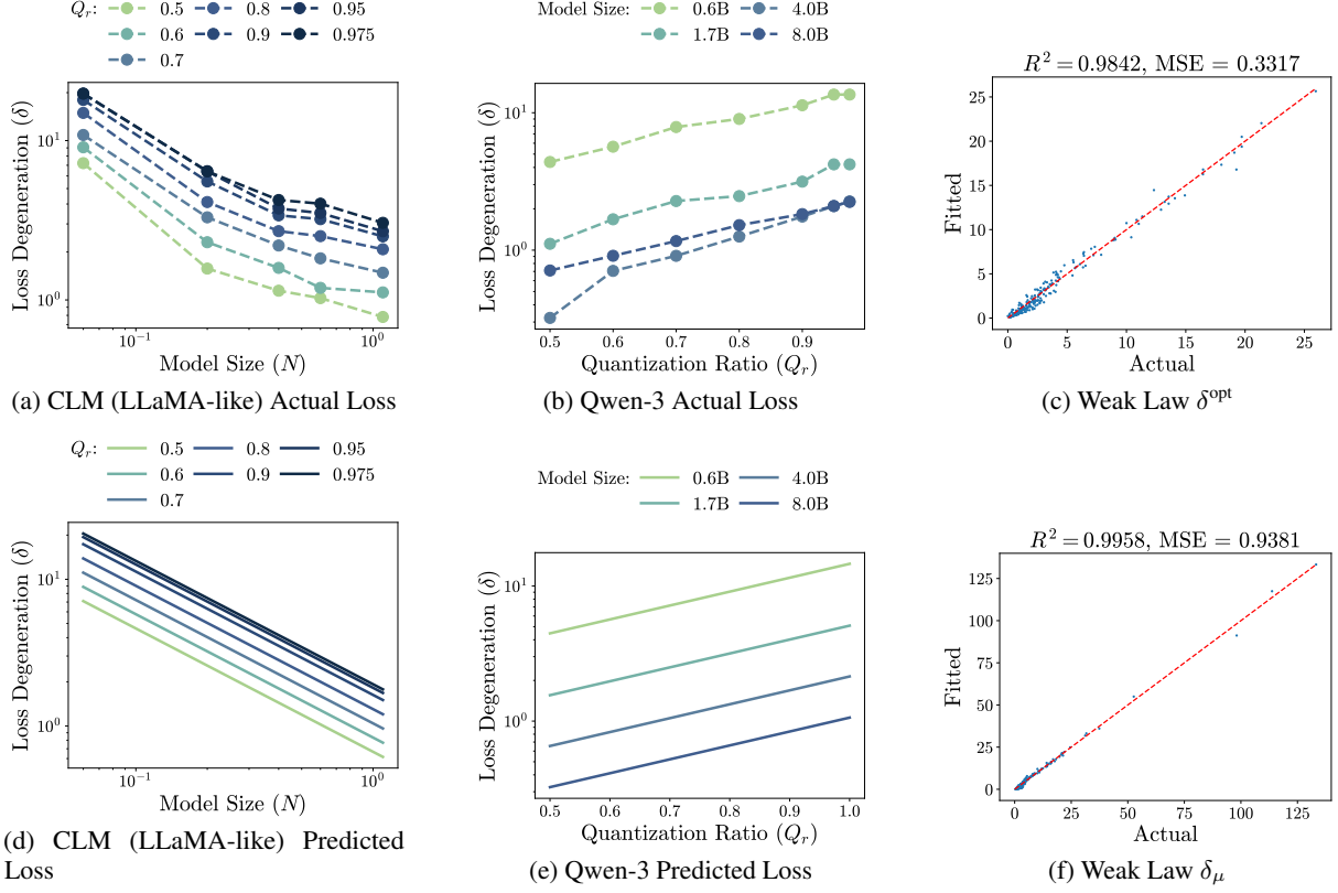
Figure 3: Weak Scaling Law Results. (a, d): Loss degradation vs. model size N for CLM, showing actual (a) and fitted (d) values. (b, e): Loss degradation vs. quantization ratio Q_r for Qwen-3, showing actual (b) and fitted (e) values. (c, f): Fitted vs. actual values for \delta^{\text{opt}} (c) and \mathbb{E}[\delta] (f) across all MXINT-4 configurations (layer-wise and matmul-wise) on CLM, Qwen-1.5, and Qwen-3. The high R^2 values in (c, f) confirm that our weak scaling law accurately captures the empirical loss degradation. Full results are in Appendices C and D.
