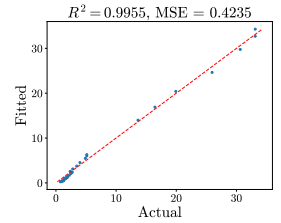
Figure 38: Minifloat Qwen-3 Weak Law. The left two are for \delta^{\text{opt}} and the right two are for \delta_\mu .
