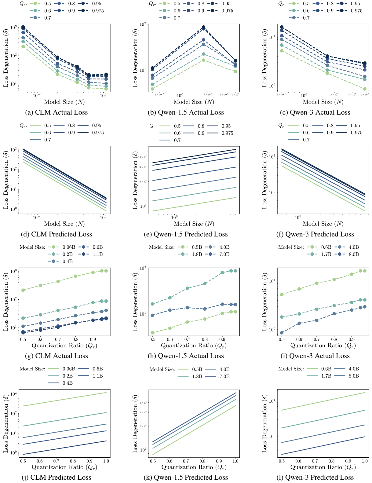
Figure 21: Minifloat ( \delta_\mu ) (a,d,g,h) CLM Minifloat results; (b,e,h,k) Qwen-1.5 Minifloat results; (c,f,i,l) Qwen-3 Minifloat results.
