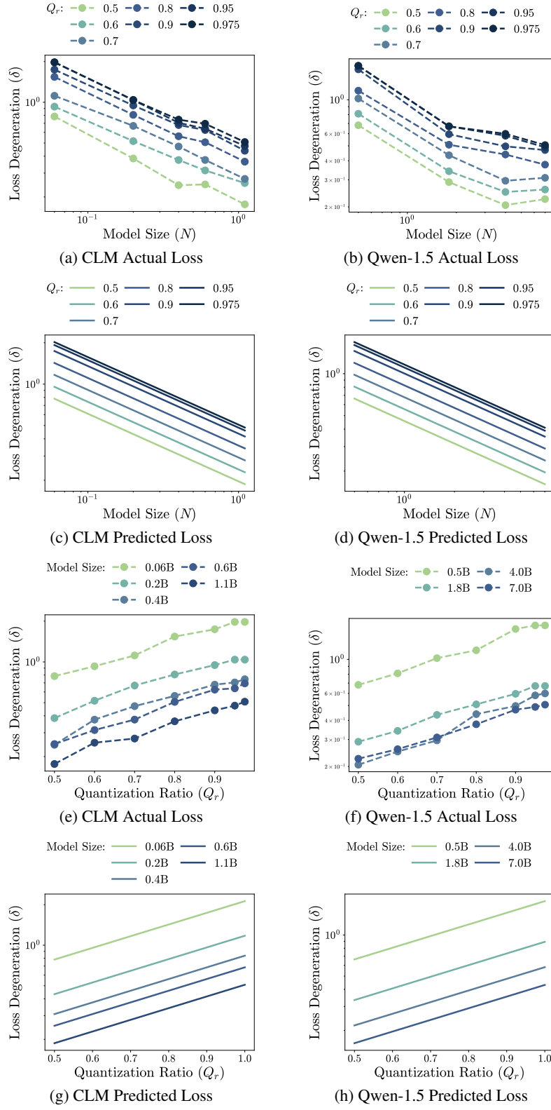
Figure 18: GPTQ ( \delta^{\text{opt}} ) (a,c,e,g) CLM GPTQ results; (b,d,f,h) Qwen-1.5 GPTQ results.
