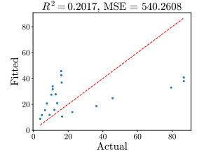
Figure 36: Minifloat CLM Weak Law. The left two are for \delta^{\text{opt}} and the right two are for \delta_\mu .
