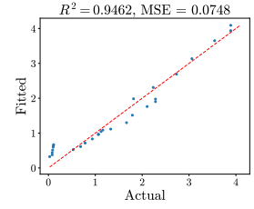
Figure 32: HQQ Qwen-1.5 Weak Law. The left two are for \delta^{\text{opt}} and the right two are for \delta_\mu .
