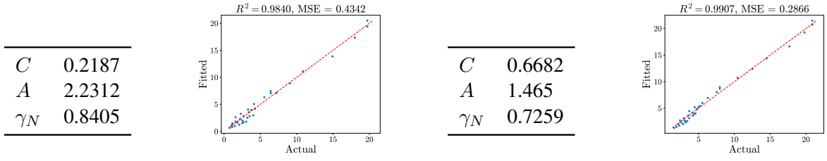
Figure 44: MXINT-2 Qwen-3 Weak Law. The left two are for \delta^{\text{opt}} and the right two are for \delta_\mu .
