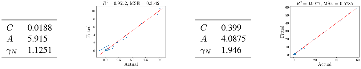
Figure 52: Weight-only MXINT-4 Qwen-1.5 Weak Law. The left two are for \delta^{\text{opt}} and the right two are for \delta_\mu .
