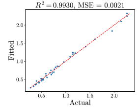
Figure 33: HQQ Qwen-3 Weak Law. The left two are for \delta^{\text{opt}} and the right two are for \delta_\mu .
