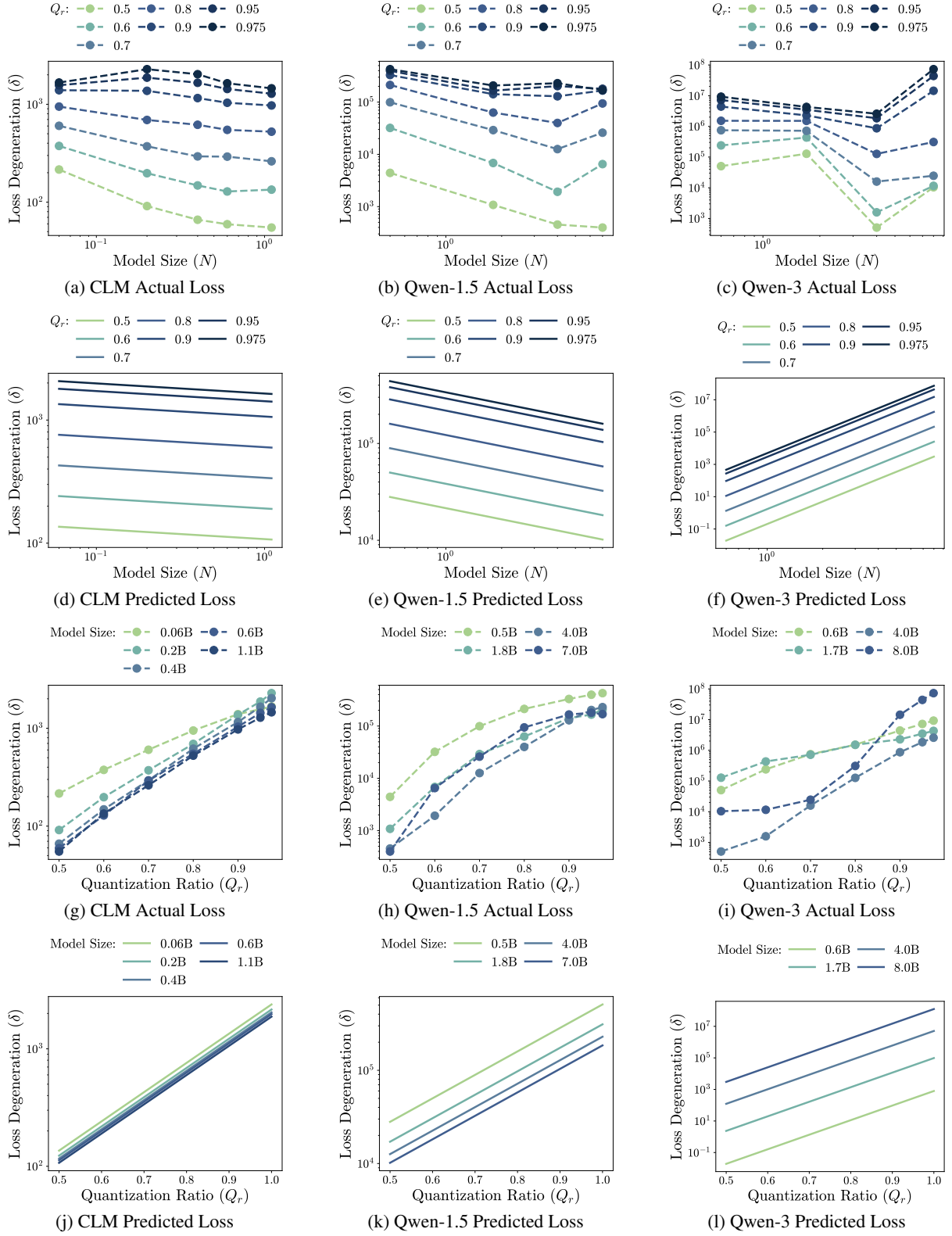
Figure 25: MXINT-2 ( \delta_\mu ) (a,d,g,h) CLM MXINT-2 results; (b,e,h,k) Qwen-1.5 MXINT-2 results; (c,f,i,l) Qwen-3 MXINT-2 results.
