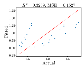
Figure 40: MXFP Qwen-1.5 Weak Law. The left two are for \delta^{\text{opt}} and the right two are for \delta_\mu .
