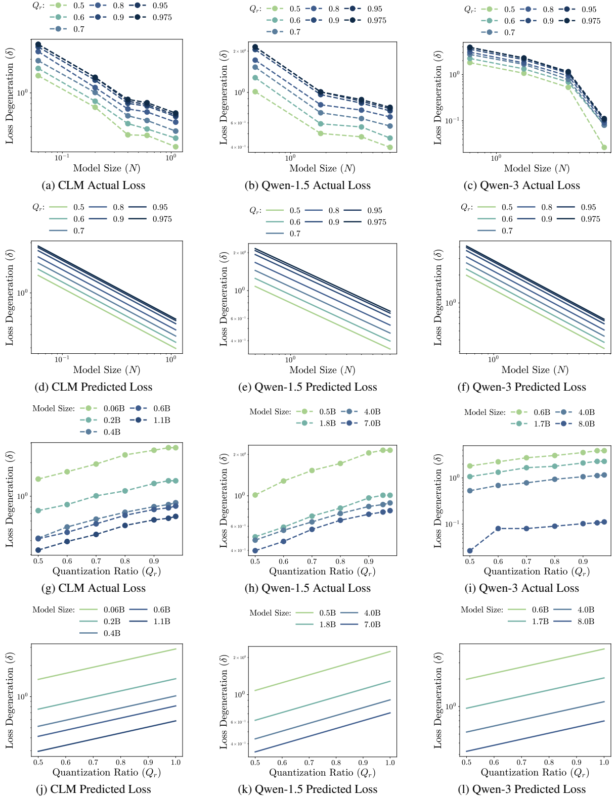
Figure 17: HQQ ( \delta_\mu ) (a,d,g,h) CLM HQQ results; (b,e,h,k) Qwen-1.5 HQQ results; (c,f,i,l) Qwen-3 HQQ results.
