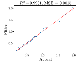
Figure 33: HQQ Qwen-3 Weak Law. The left two are for \delta^{\text{opt}} and the right two are for \delta_\mu .
