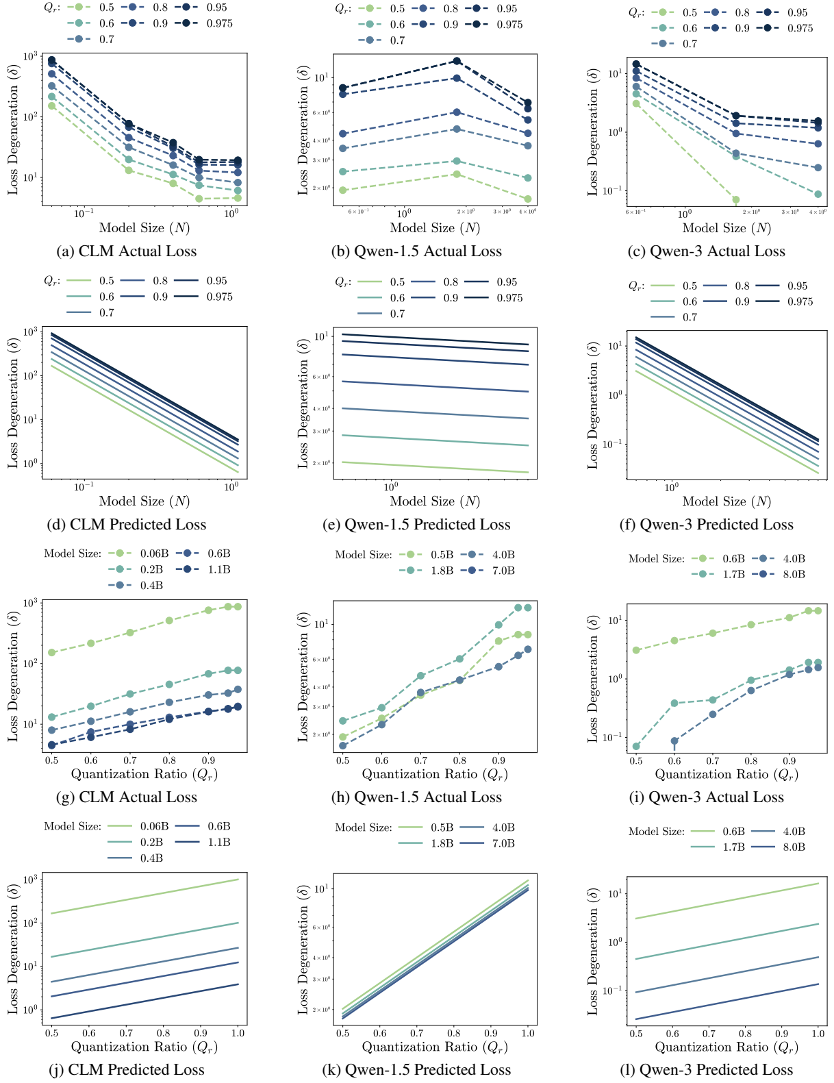
Figure 20: Minifloat ( \delta^{\text{opt}} ) (a,d,g,h) CLM Minifloat results; (b,e,h,k) Qwen-1.5 Minifloat results; (c,f,i,l) Qwen-3 Minifloat results.
