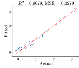
Figure 32: HQQ Qwen-1.5 Weak Law. The left two are for \delta^{\text{opt}} and the right two are for \delta_\mu .
