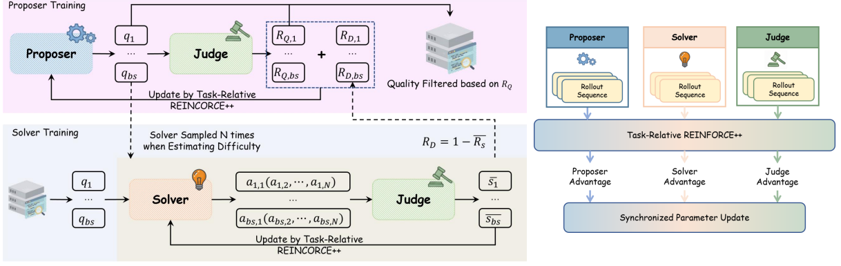
Figure 2: Multi-Agent Evolve Framework: (Left) In Multi-Agent Evolve, Proposer generates questions and receive reward based on Judge evaluation and difficulty estimation. After applying quality filter on the generated questions, only a portion of the questions enter the maintained dataset for future usage. For the Solver, it receives the Judge’s evaluation as well. (Right) Our multi-agent training employs Task-Relative REINFORCE++, which computes the advantage for each role separately and then performs a synchronized parameter update to the uniform model.
