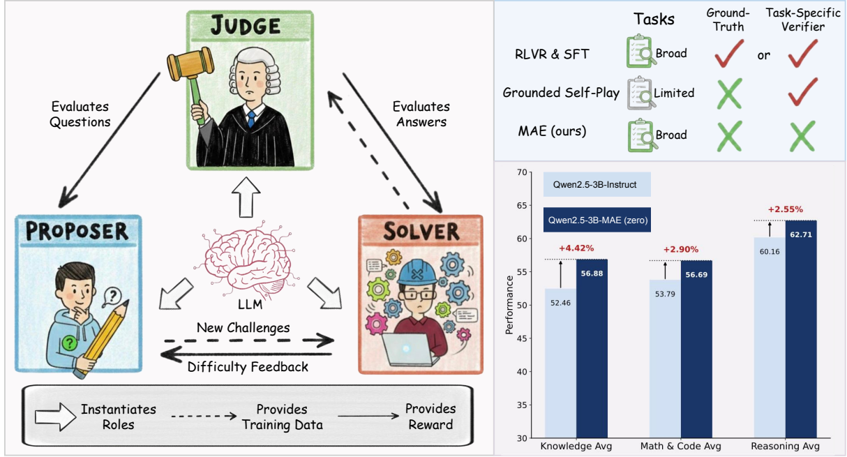
Figure 1: Overview of Multi-Agent Evolve (MAE). (Top Right) Comparison with existing training paradigms: unlike Reinforcement Learning with Verifiable Rewards (RLVR) and SFT which rely on expensive human data or task-specific verifiers, and grounded self-play RL which is limited to tasks with ground-truth simulators, MAE scales to broad tasks without external supervision. (Left) The MAE framework instantiates three interactive roles ( Proposer , Solver , and Judge ) from a single LLM to form a closed self-improving loop. The Proposer generates new challenges, the Solver attempts to answer them, and the Judge evaluates the output. This creates an adversarial co-evolution process where the Proposer is incentivized by difficulty feedback to create harder questions as the Solver improves. (Bottom Right) MAE (zero) enhances the performance of Qwen2.5-3B-Instruct across Knowledge QA, Math & Code, and Reasoning benchmarks with no human supervision.
