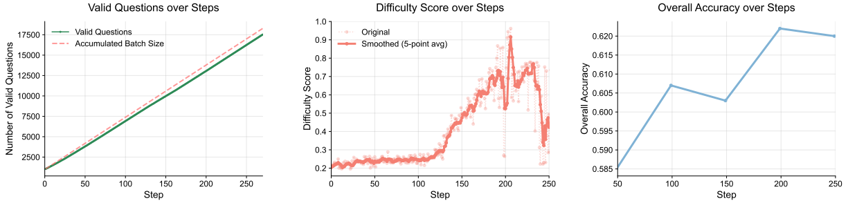
Figure 3: Training Process Analysis: These three figures demonstrate an example training process. (Left) The number of questions in the dataset increases steadily while low-quality questions are excluded. (Mid and Right) The Proposer learns to generate questions that present a desirable level of difficulty to the Solver, thereby benefiting the model in future training.
