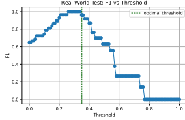
Figure 22: Real World: F1 vs. Threshold
