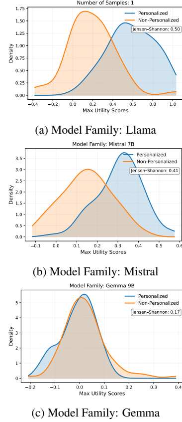
Figure 6: Distribution of maximum utility scores for a personalized (blue) and non-personalized (orange) dataset calculated using models of different families.
