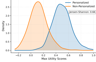
Figure 2: Distribution of maximum utility scores for personalized (PersonaFeedback) and non-personalized (FreebaseQA) inputs. Personalized inputs exhibit substantially higher utility scores, indicating stronger sensitivity to user memory.
