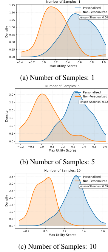
Figure 10: Distribution of maximum utility scores for a personalized (blue) and non-personalized (orange) dataset differing number of Monte Carlo samples average over.
