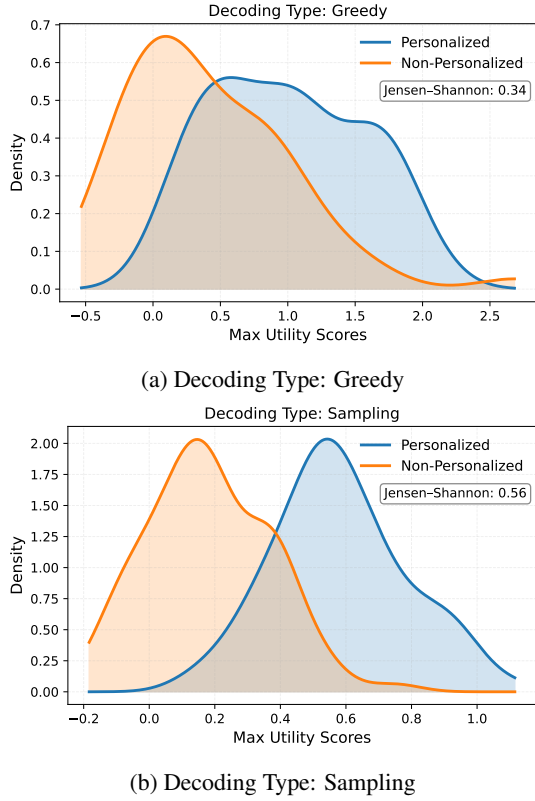
Figure 7: Distribution of maximum utility scores for a personalized (blue) and non-personalized (orange) dataset differing by decoding type.
