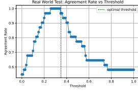
Figure 20: Real World: % Agreement vs. Threshold
