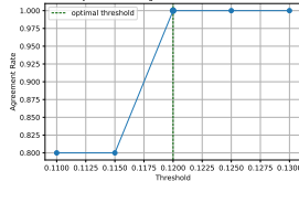
Figure 17: Synthetic: % Agreement vs. Threshold (zoomed in)
