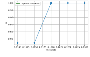
Figure 19: Synthetic: F1 vs. Threshold (zoomed in)
