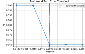
Figure 23: Real World: F1 vs. Threshold (zoomed in)
