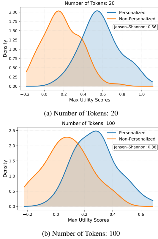
Figure 9: Distribution of maximum utility scores for a personalized (blue) and non-personalized (orange) dataset using different number of tokens.
