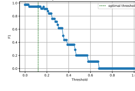
Figure 18: Synthetic: F1 vs. Threshold
