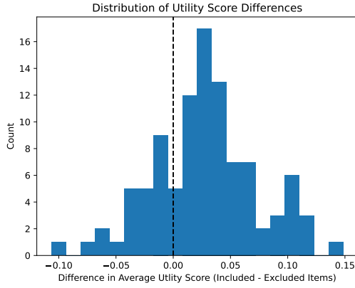
Figure 14: RUMS-Binary: Difference
