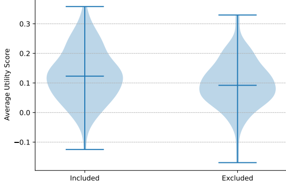
Figure 12: RUMS-Binary: Distribution
