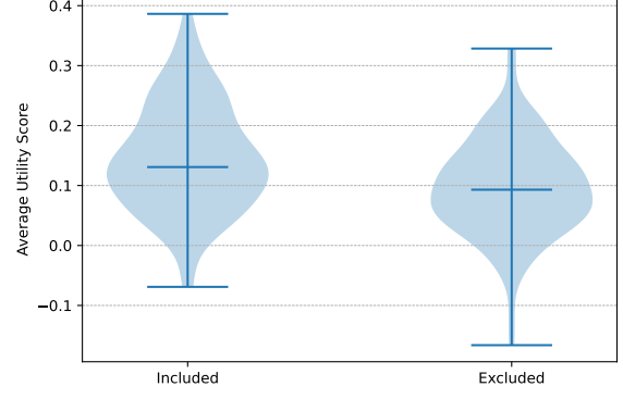
Figure 13: RUMS-Multi: Distribution
