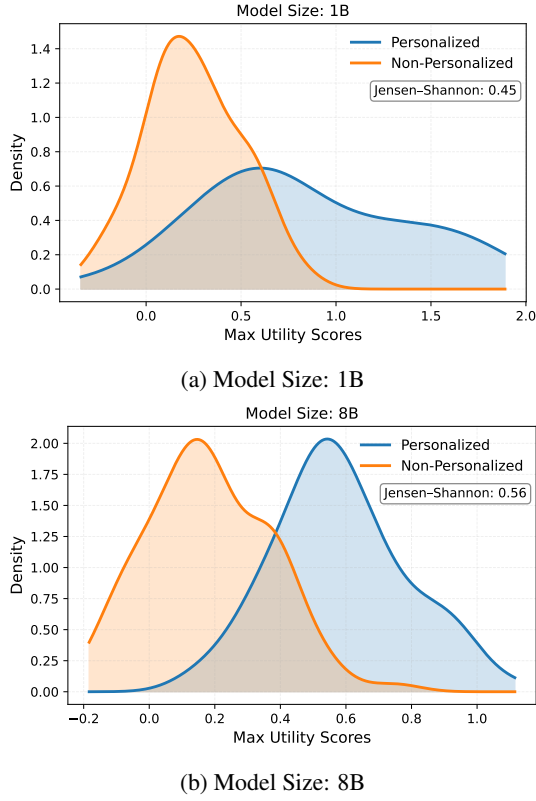
Figure 5: Distribution of maximum utility scores for a personalized (blue) and non-personalized (orange) dataset differing by size of model used for entropy calculation.
