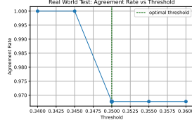
Figure 21: Real World: % Agreement vs. Threshold (zoomed in)
