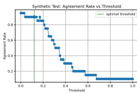
Figure 16: Synthetic: % Agreement vs. Threshold
