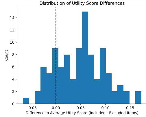
Figure 15: RUMS-Multi: Difference
