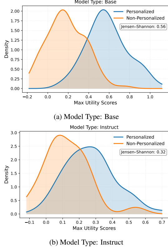
Figure 4: Distribution of maximum utility scores for a personalized (blue) and non-personalized (orange) dataset differing by type of model used for entropy calculation.
