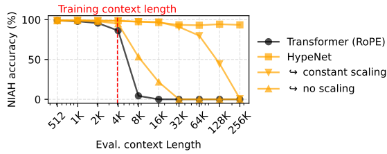
Figure 8: Results for validating attention logits scaling (see Eq. 11). The plot shows the NIAH performance of HypeNet without attention logits scaling, HypeNet with constant scaling (which is common in RoPE-based length extrapolation methods), and HypeNet with the attention logits scaling defined in Eq. 11.
