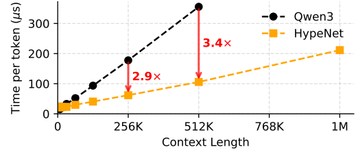
Figure 6: The prefilling time of HypeNet versus Qwen3-1.7B, across different context lengths.
