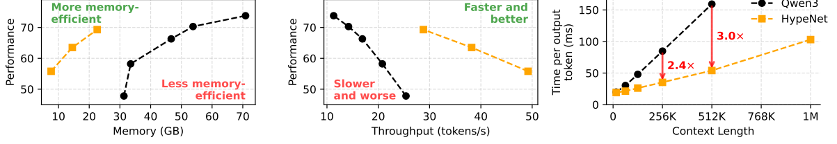
Figure 1: Left & center: the performance-efficiency tradeoff of HypeNet (ours), versus the Qwen3 series, measured with 128K context length and BFloat16 precision. Right: the time per output token of the 1.7B models across different context lengths. At 1M context length, Qwen3 runs out of GPU memory. HypeNet is converted from Qwen3 using our distillation procedure, HALO, and has better performance-efficiency tradeoff than Qwen3.
